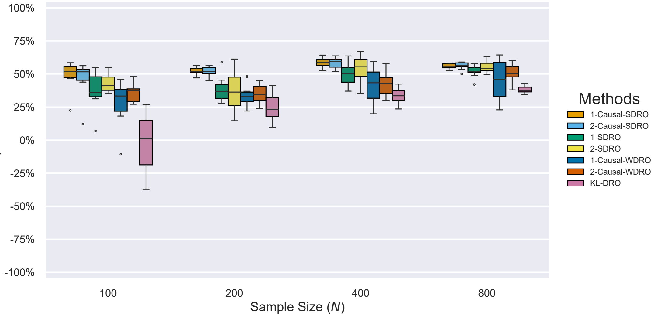
Out-of-sample Performance
