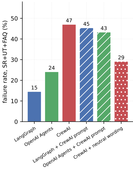
qwen2.5 7B (local)
