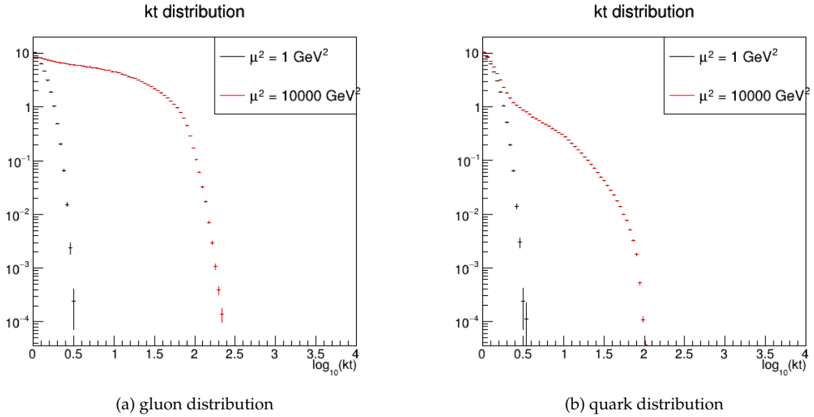
Figure 2.3: Evolution of the transverse momentum distribution.
