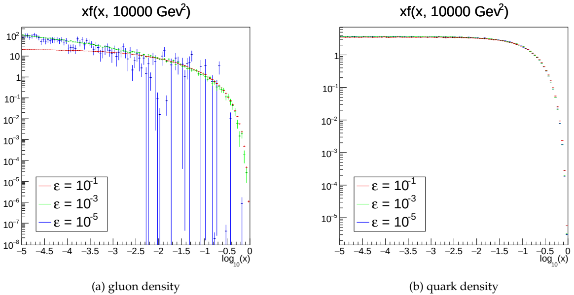
Figure 2.5: Evolved momentum weighted parton density, depending on \epsilon .
