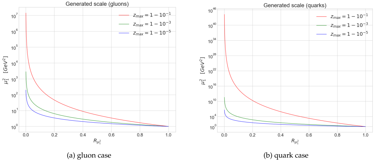
Figure 2.9: First generated scale \mu_1^2 with respect to R_{\mu_1^2} , fixed z_{min} , variable z_{max} .
