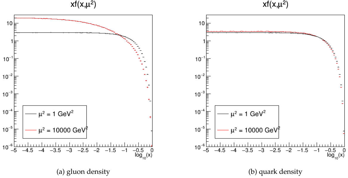
Figure 2.2: Evolution of the momentum weighted parton density.
