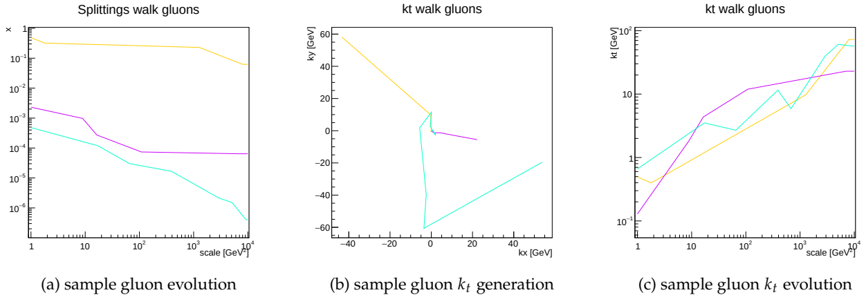
Figure 2.1: Evolution process for a sample of three gluon.
