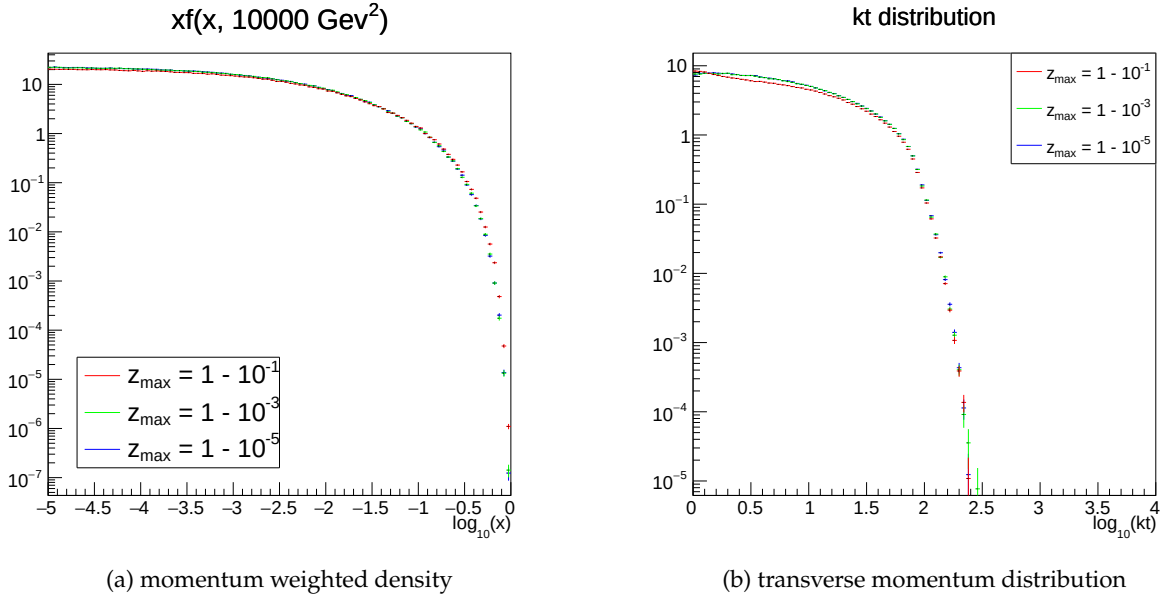
Figure 2.11: Evolved gluon densities, fixed z_{min} , variable z_{max} .
