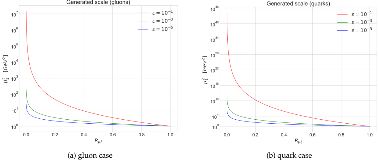
Figure 2.4: First generated scale \mu_1^2 with respect to the random number R_{\mu_1^2} , depending on \epsilon .
