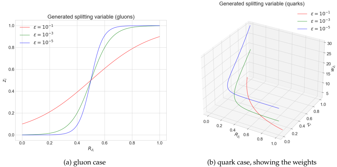
Figure 2.7: Generated splitting variable z_i with respect to the random number R_{z_i} , depending on \epsilon .
