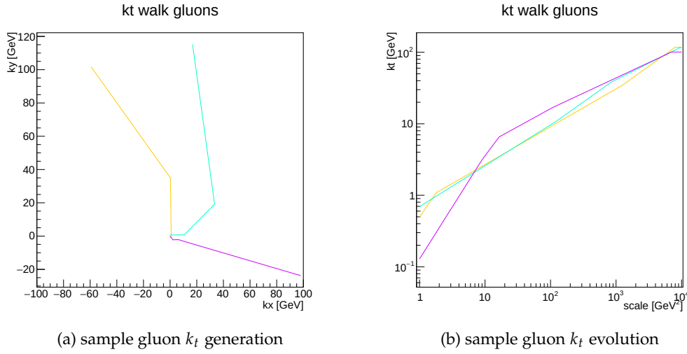
Figure 2.12: k_t evolution with transverse ordering, for a sample of three gluons, z_{max} = 0.9 .
