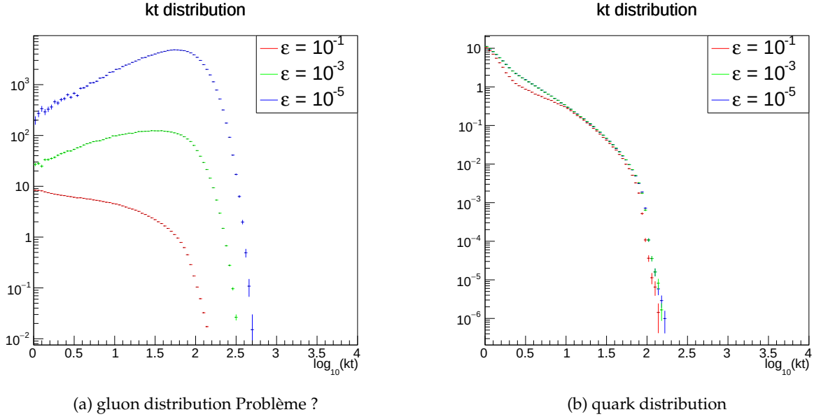
Figure 2.6: Evolved transverse momentum distribution, depending on \epsilon .
