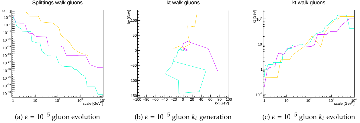
Figure 2.8: Evolution process for a sample of three gluon, with \epsilon = 10^{-5} .
