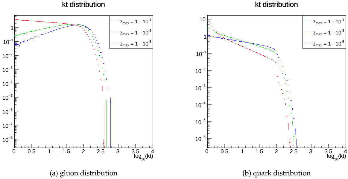
Figure 2.13: Evolved k_t distribution, transverse ordering, variable z_{max}
