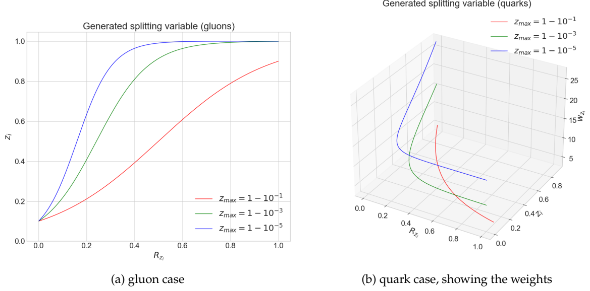
Figure 2.10: Generated splitting variable z_i with respect to R_{z_i} , fixed z_{min} , variable z_{max} .
