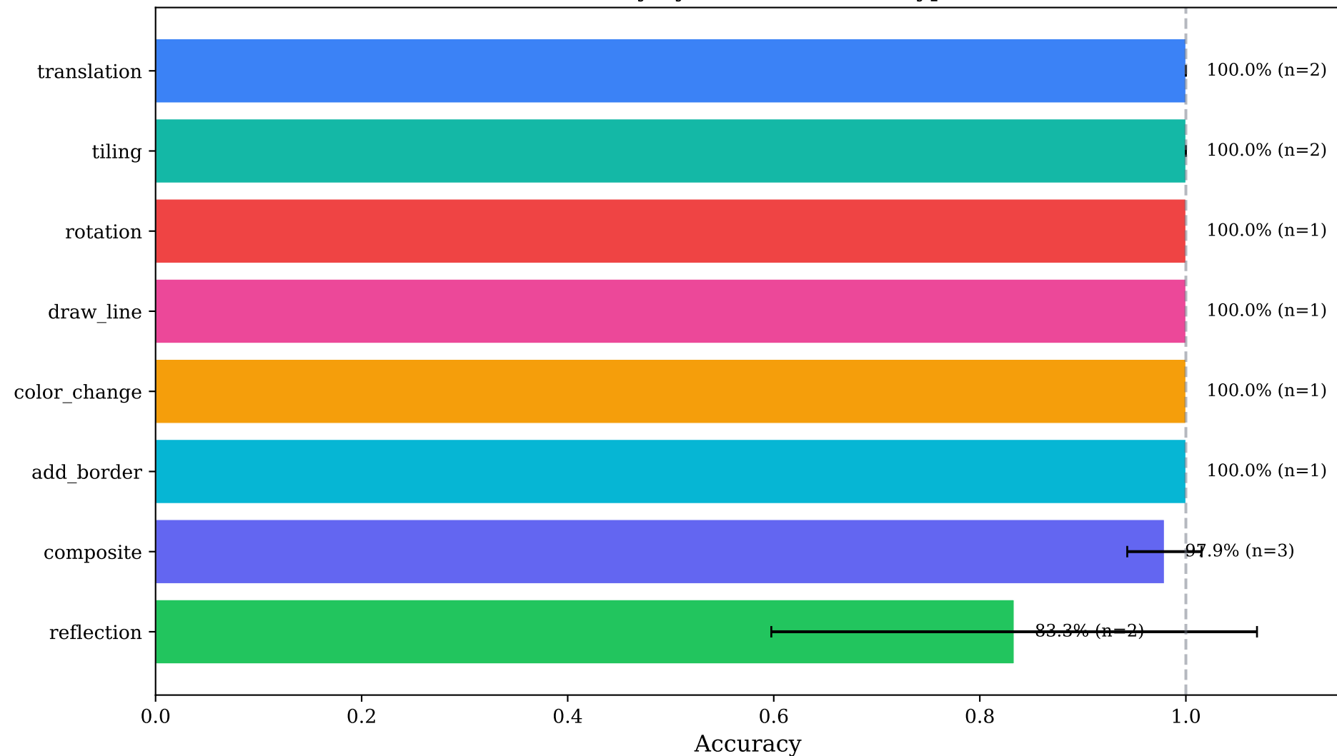
Accuracy by Transformation Type
