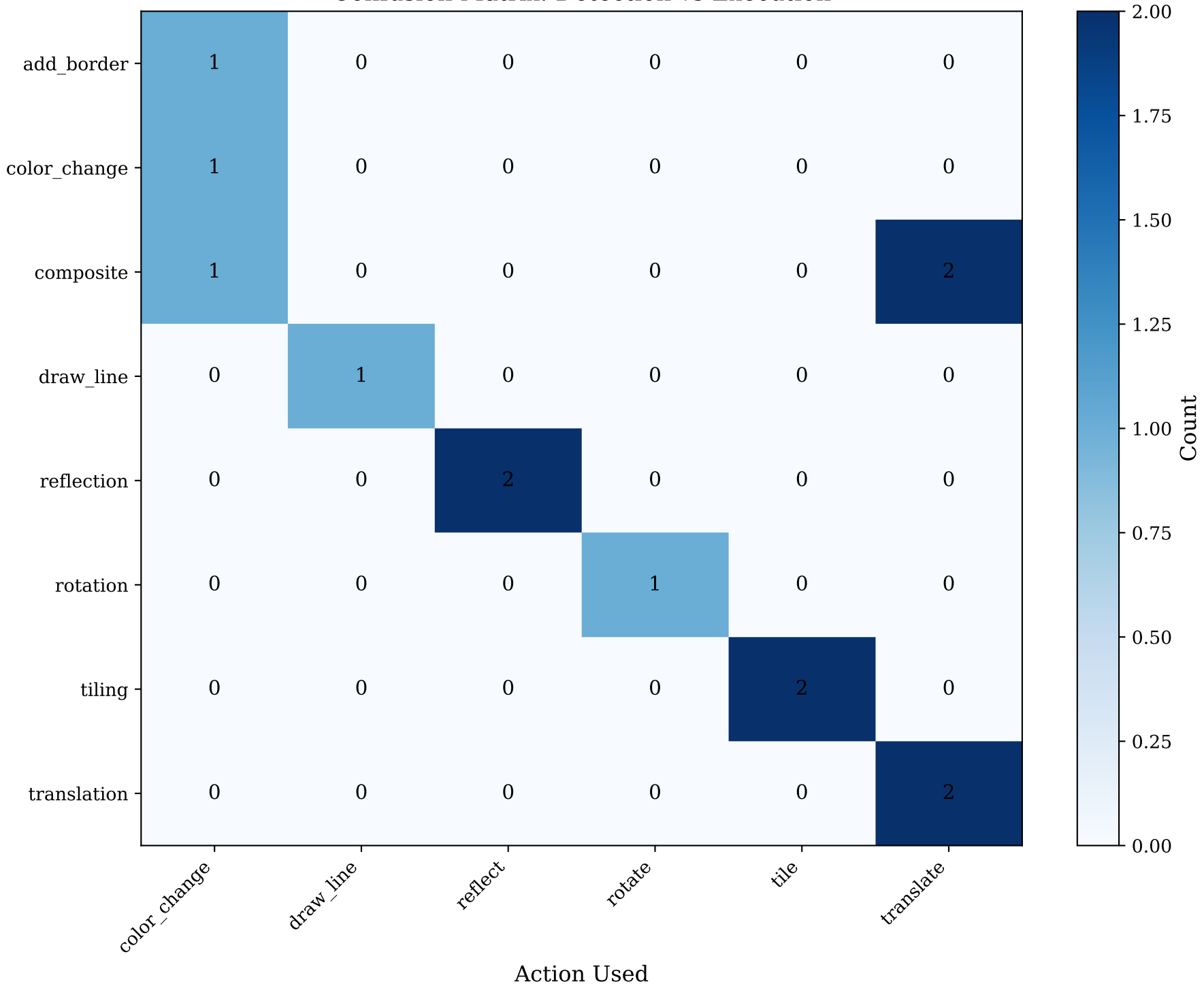
Confusion Matrix: Detection vs Execution
