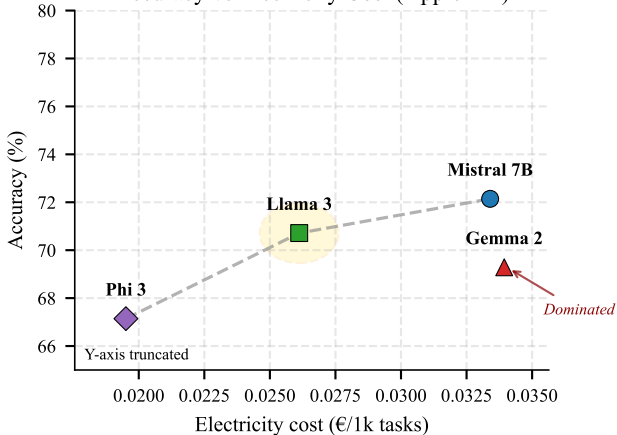
Accuracy vs Electricity Cost (Apple M1)
