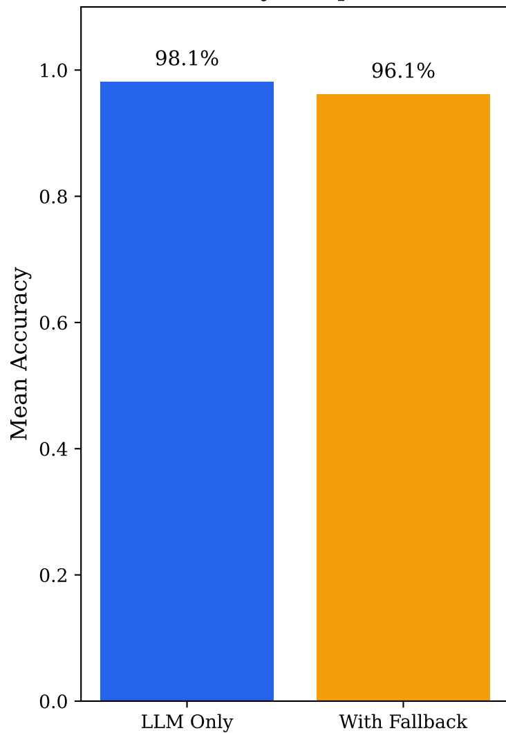
Accuracy Comparison
