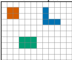
Train 2 input
