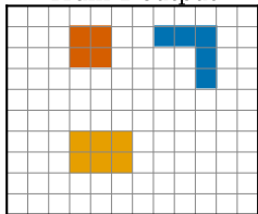
Train 2 output
