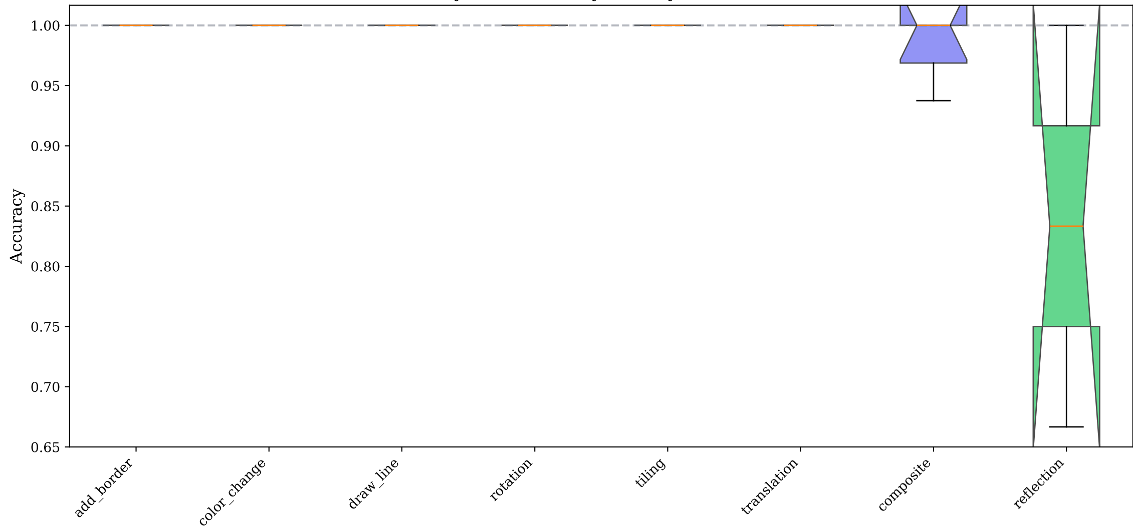
Accuracy Distribution by Primary Transformation
