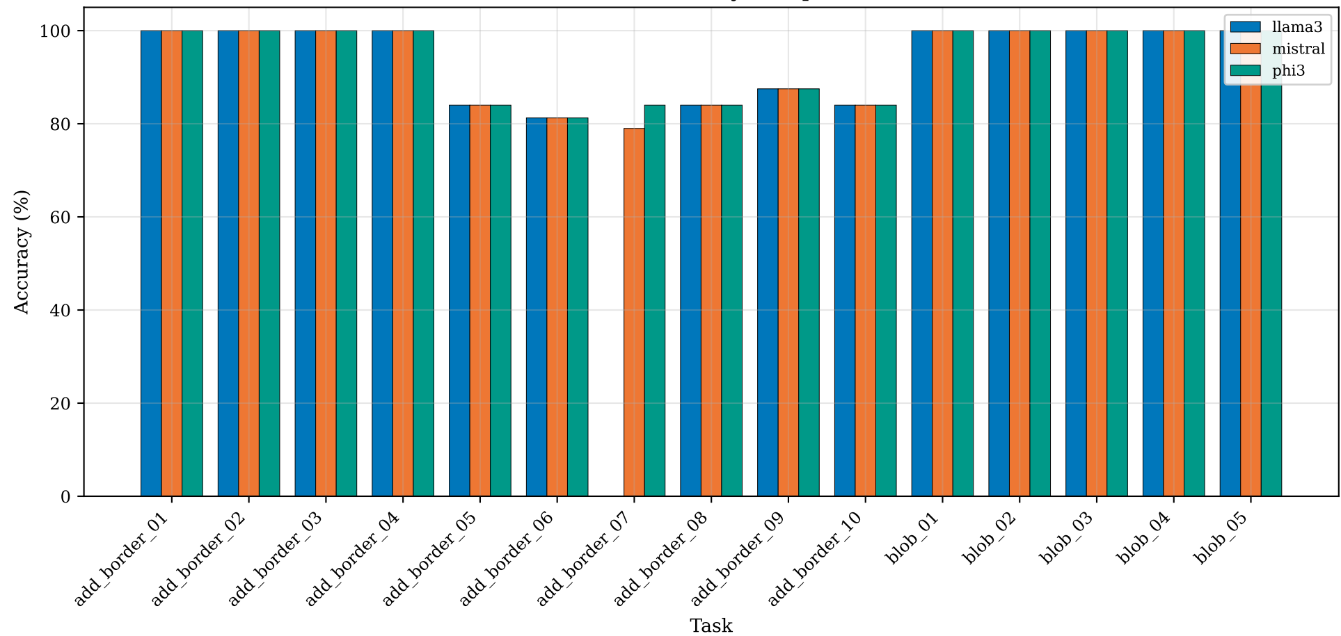
Per-Task Accuracy Comparison
