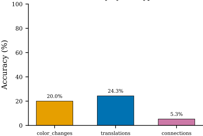
Accuracy by rule type
