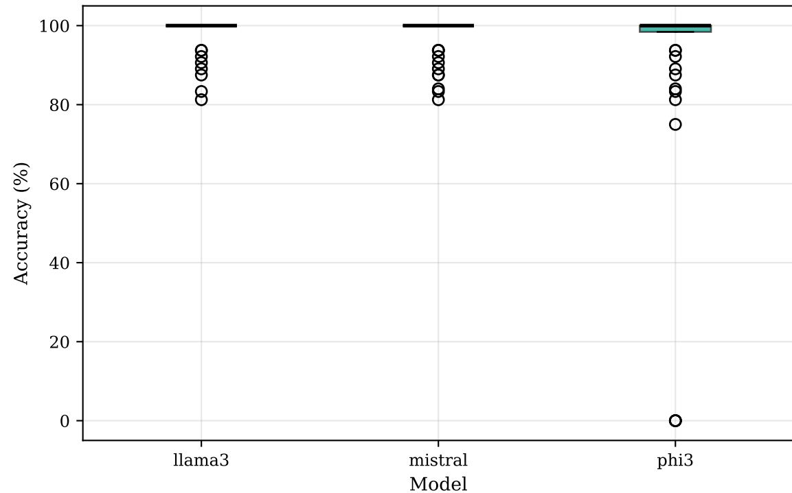
Accuracy Distribution by Model
