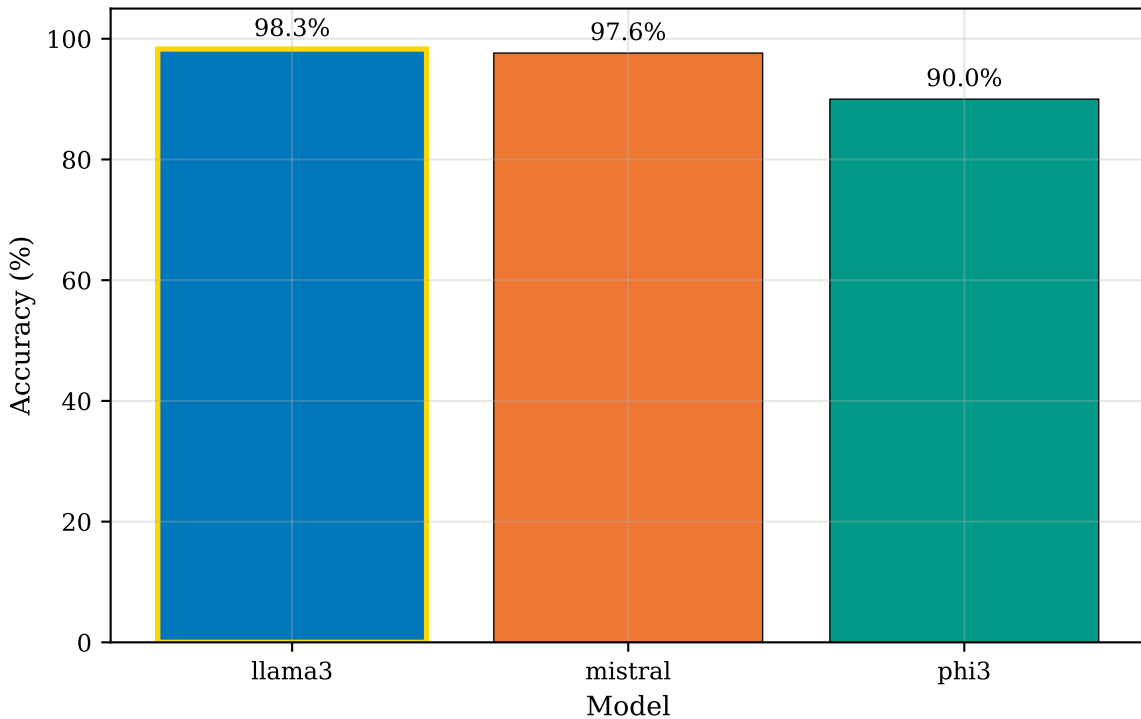
Model Accuracy Comparison (n=52 tasks)
