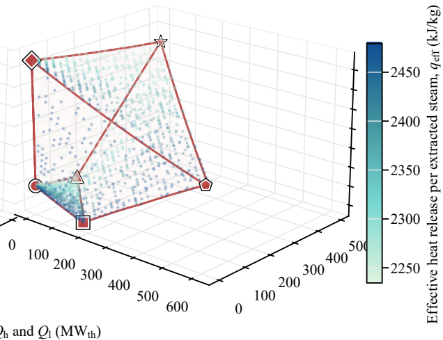
(b) C3 source feasible domain
