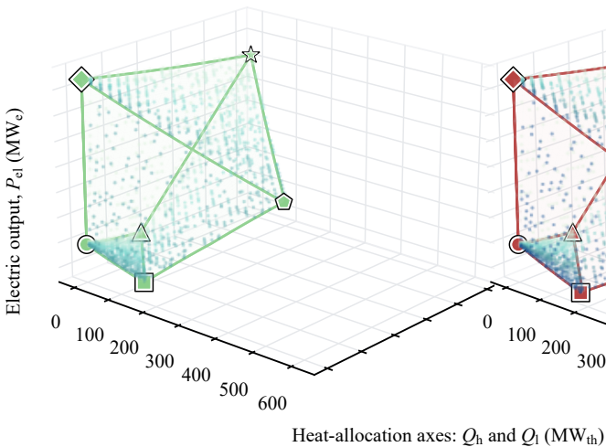
(a) C2 source feasible domain
