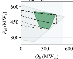
(c) Q_{\text{h}} \text{--} P_{\text{el}}
