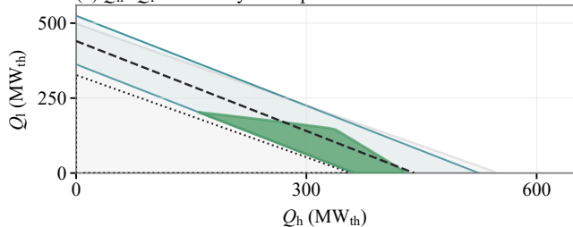
(b) Q_{\text{h}} \text{--} Q_{\text{l}} : DHN-only vs coupled
