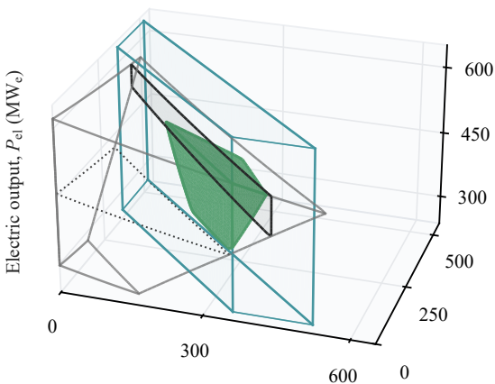
(a) C2: fixed DHN condition, T_{\text{amb}} = -10\text{ }^{\circ}\text{C}
