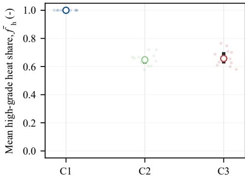
(a) Heat-grade allocation
