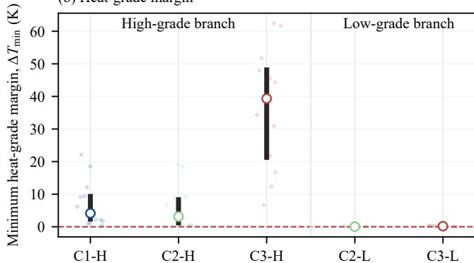
(b) Heat-grade margin
