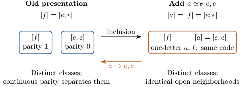
FIGURE 7. A primitive-to-word substitution preserves the presented algebra but can change the observable topology (Proposition 5.5). Adding the defining rule gives inverse scoped substitutions. Inclusion is continuous on the observable quotient; elimination is discontinuous because it sends inseparable classes to classes separated by parity. Boxes indicate separation properties, not asserted open two-point subspaces.
