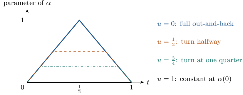
FIGURE 4. Backtracking cancellation as an explicit homotopy. The plotted function is r_u(t) = \min\{2t, 2(1-t), 1-u\} ; the actual path is H(u, t) = \alpha(r_u(t)) . As u increases, the turning point retreats along \alpha and the path waits there before returning. All intermediate paths stay in \alpha(I) , so even a hole surrounded by \alpha cannot obstruct this cancellation.
