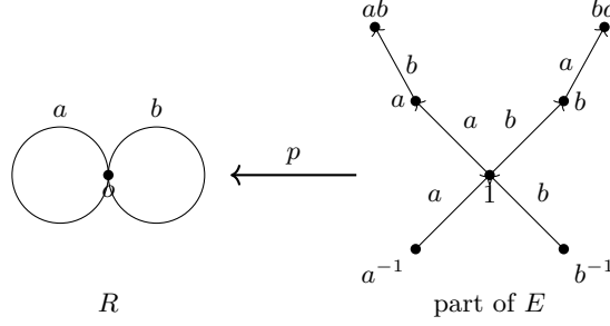
FIGURE 11. The geometric covering records word order in lifted endpoints. The two words ab and ba end at different vertices above the same basepoint. The pictured finite part belongs to the full interval-glued Cayley realization.
