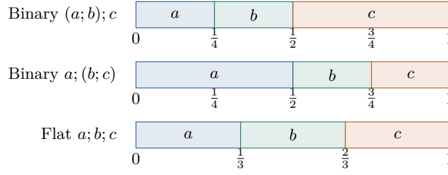
FIGURE 6. Exact timing depends on the trace model. Recursive binary concatenation halves each concatenation interval; equal-slot realization assigns one third to each letter of this word, independently of parentheses. Homotopy between these paths does not identify topologies that observe their exact parametrizations.
