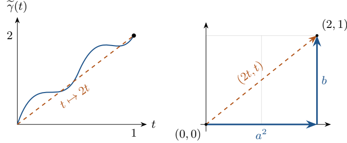
FIGURE 10. Winding separates normal forms because lifts remember endpoints. Left: a lift beginning at 0 and ending at 2 is straightened to 2t . Right: the sequential word a^2; b and the simultaneous loop have lifts with common endpoints (0,0) and (2,1) ; straight-line interpolation in \mathbb{R}^2 gives a homotopy after projection to the torus. Both plots are drawn in the covering spaces \mathbb{R} and \mathbb{R}^2 .
