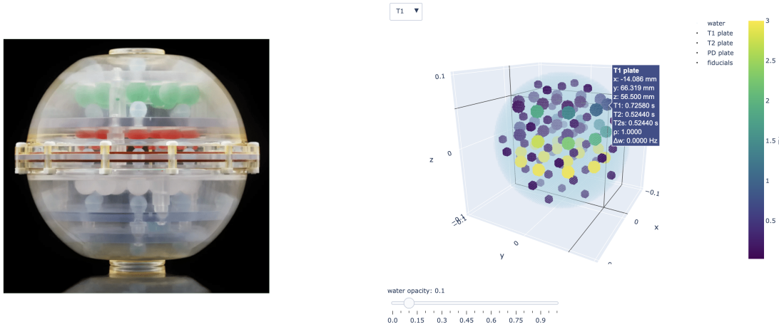
Figure 3.1: The QalibreMD NIST/ISMRM System Standard Model 130 hardware phantom and its digital T1 array. The physical phantom photo (left) is reproduced from Caliber MRI. The voxelised plot of the digital phantom (right), coloured by T1 value, can be reproduced by running examples/plot_phantom_3d.jl in MRISystemPhantom .
