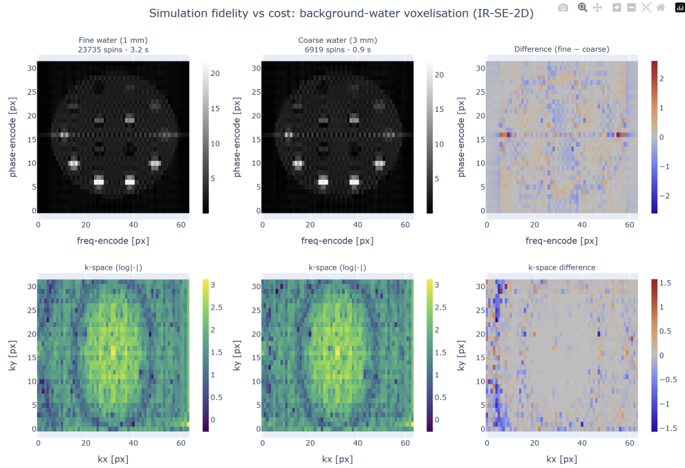
Figure 3.2: Fidelity–cost trade-off of background-water voxelisation. The same IR-SE-2D acquisition ( TI/TE/TR = 400/80/1500 ms, 32 \times 64 , FOV 0.2 m) is simulated through two phantoms differing only in background-water discretisation. Top row: magnitude images; bottom row: log-magnitude k-space; right column: fine - coarse difference. The figure and numbers are reproduced by examples/compare_water_coarseness.jl .
