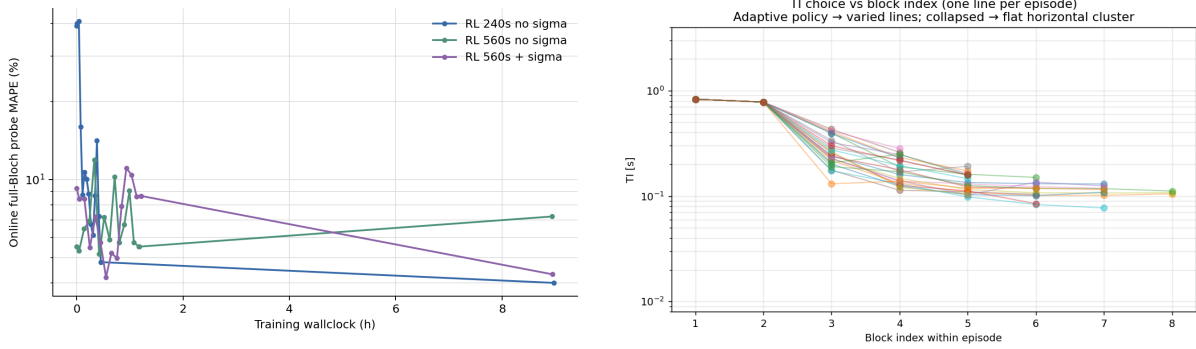
Figure 5.3: Run B 240 s policy behaviour. Left: full-Bloch probes during the curriculum. The final full stage is noisy and global-best selection is needed. Right: the global-best policy opens with a high-TI probe and then uses shorter adaptive refinements.
