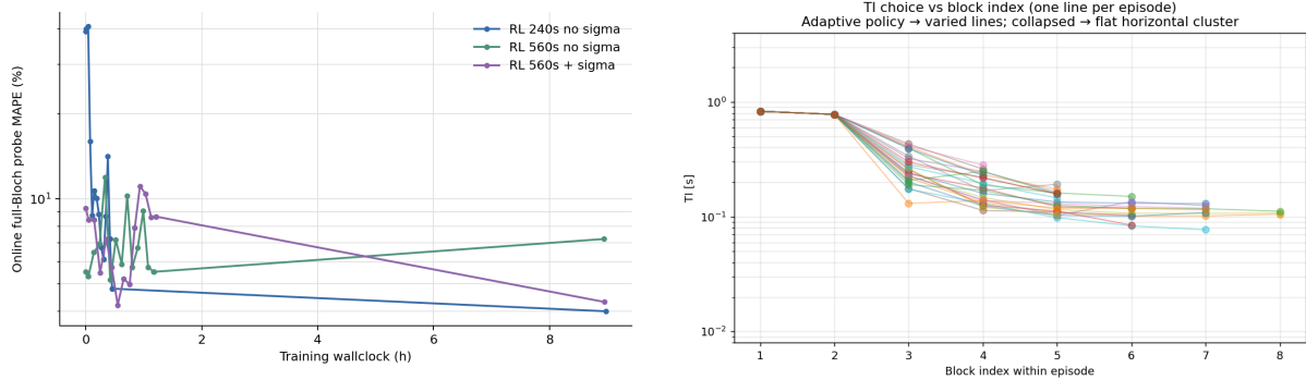
Figure 5.5: Run B 240 s policy behaviour. Left: full-Bloch probes during the curriculum. The final full stage is noisy and global-best selection is needed. Right: the global-best policy opens with a high-TI probe and then uses shorter adaptive refinements.
