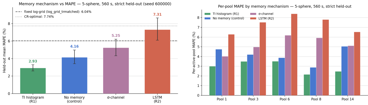
Figure 5.6: Memory ablation on the strict held-out evaluation. Left: mean MAPE with 95% CIs per memory mechanism; horizontal lines mark the fixed schedules on the same seed. Right: per-active-pool MAPE. The histogram arm is the best arm on every pool, including the long- T_1 pool that no 14-sphere policy solved.
