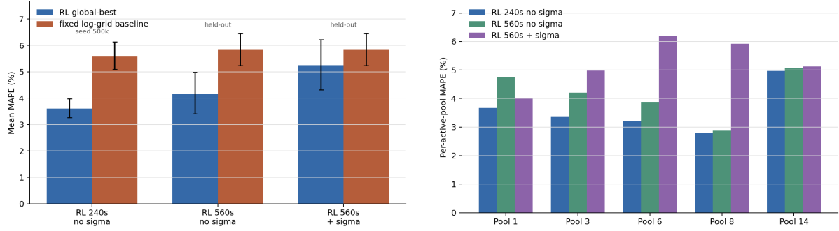
Figure 5.4: Run B five-sphere results. Left: global-best RL policies compared with the matched fixed log-grid baseline (240 s bars: selection-stream seed; Table 5.6 adds the strict held-out confirmation; 560 s bars: strict held-out evaluation). Right: per-active-pool MAPE for the RL policies.
