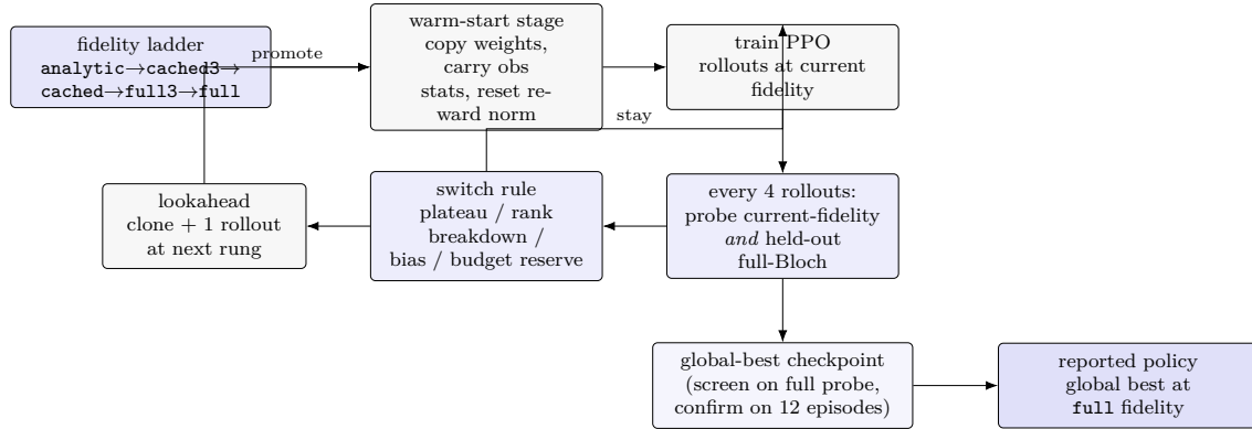
Figure 5.2: Overall logic of the multi-fidelity RL training. One PPO policy is warm-started up the fidelity ladder. While a stage trains, it is probed every four rollouts on both the current (cheap) fidelity and a held-out full-Bloch environment; the switch rule promotes to the next rung when the cheap rung is exhausted or stops tracking the full simulator, optionally confirmed by a one-rollout lookahead clone at the next rung. Crucially, promotion and checkpoint selection are driven by the full-simulator probe, never the cheap rung’s own score, so a biased rung cannot certify its own policy. The global-best checkpoint (screened on the probe, confirmed on twelve episodes) at the final full fidelity is the reported policy.
