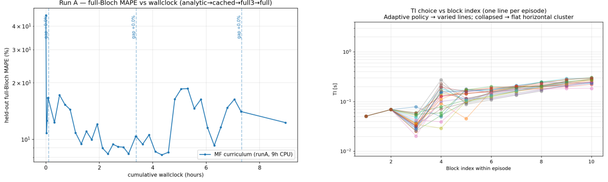
Figure 5.3: Run A curriculum behaviour. Left: full-Block probe MAPE versus wall-clock time. The cached-water stage reached the best basin, then full3 regressed. Right: the learned policy was not collapsed; TI varies across episodes and within an episode, but the final policy still under-sampled the long- T_1 regime.
