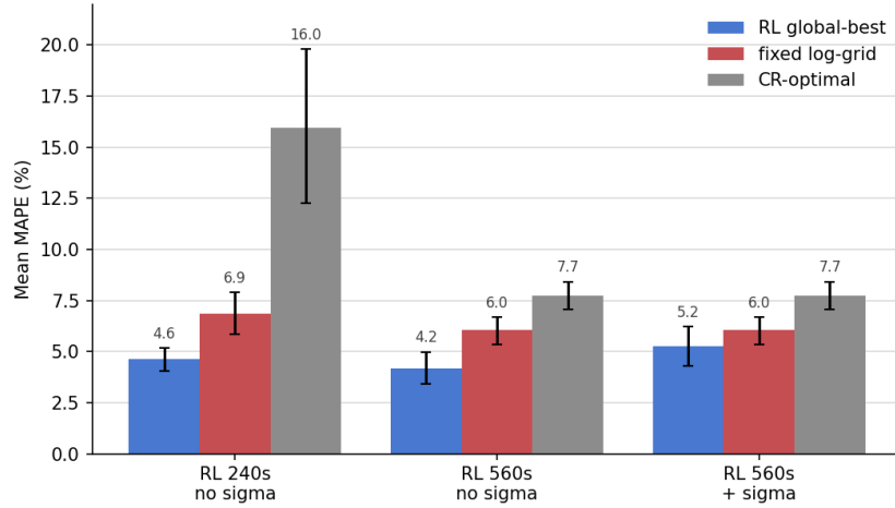
Figure 5.4: Run B five-sphere results, all on the held-out seed: global-best RL policies versus the matched fixed log-grid and CR-optimal baselines at 240 s and 560 s, plus the \sigma -channel memory arm. The CR-optimal schedule collapses at 240 s because it is solved for one nominal fleet (Section 5.6).
