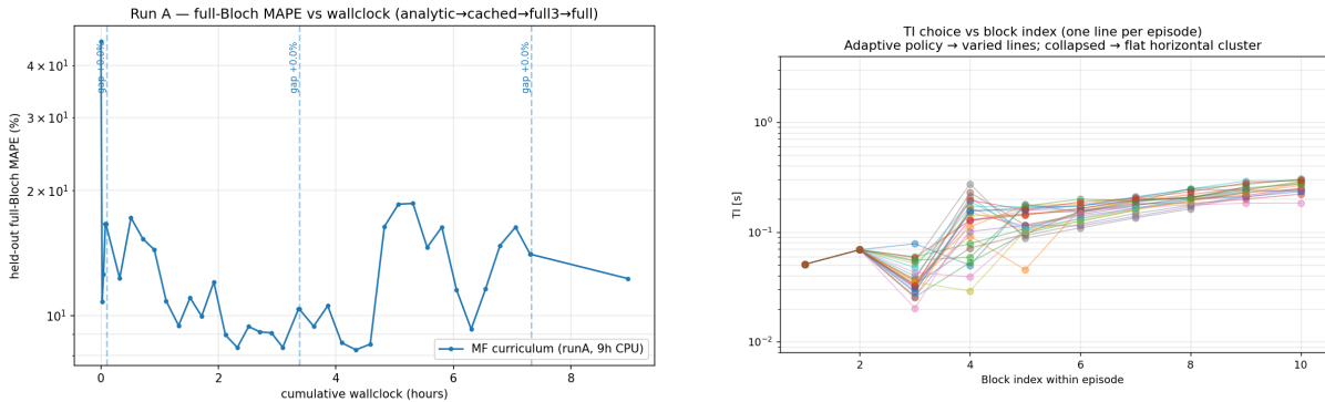
Figure 5.3: Run A curriculum behaviour. Left: full-Bloch probe MAPE versus wall-clock time. The cached-water stage reached the best basin, then full3 regressed. Right: the learned policy was not collapsed; TI varies across episodes and within an episode, but the final policy still under-sampled the long-T1 regime.
