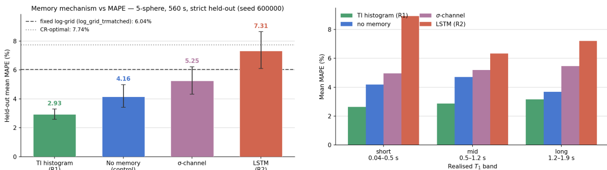
Figure 5.6: Memory ablation on the strict held-out evaluation. Left: mean MAPE with 95% CIs per mechanism; horizontal lines mark the fixed schedules on the same seed. Right: mean MAPE binned by realised T_1 (the meaningful breakdown, since each sphere is an independent draw), showing the histogram arm is the most accurate in every band.
