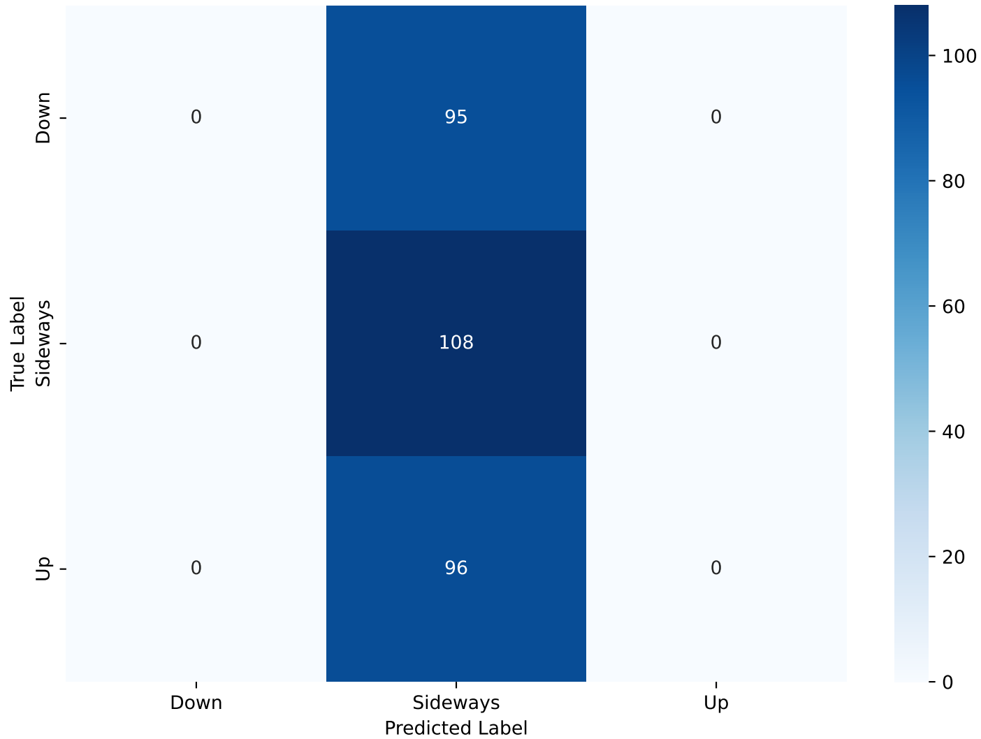
QLSTM_OHLCV_Classification - Confusion Matrix
