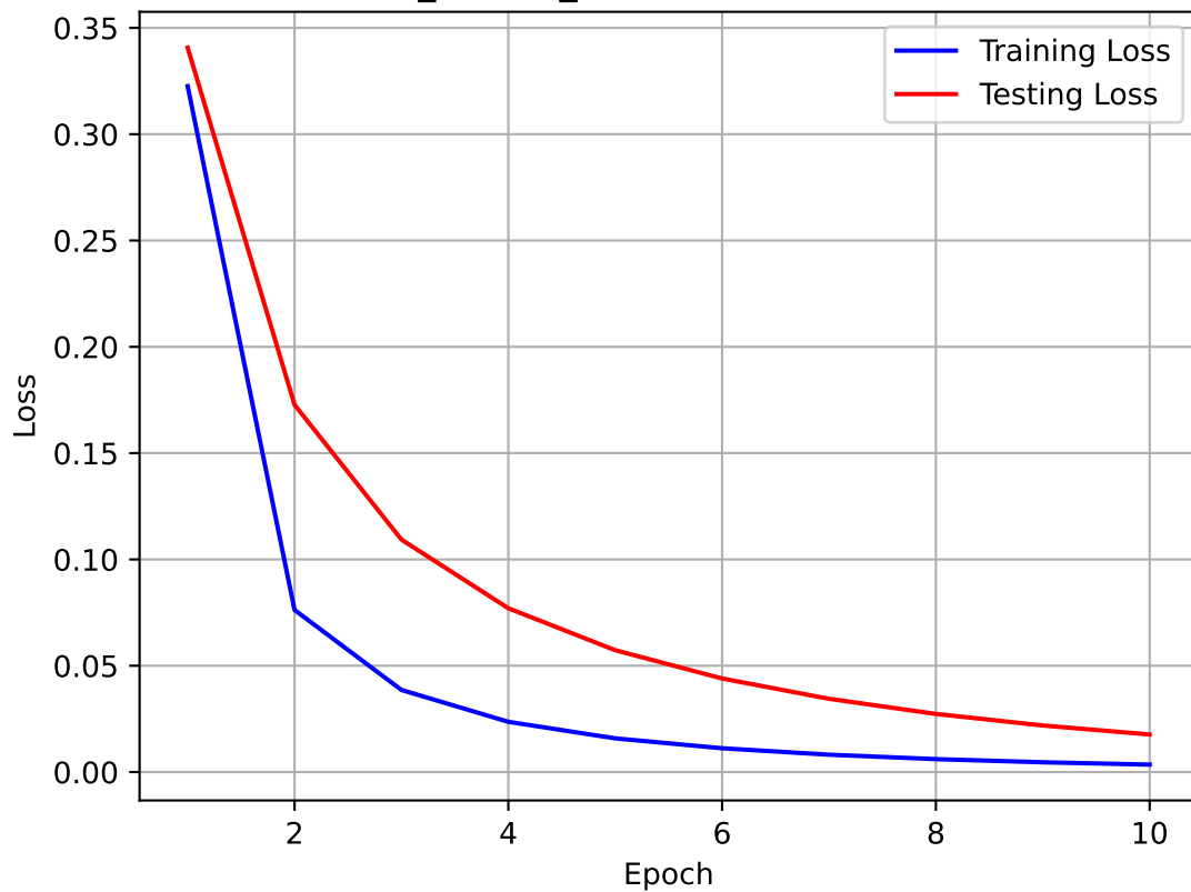
QLSTM_OHLCV_Classification - Loss Curve
