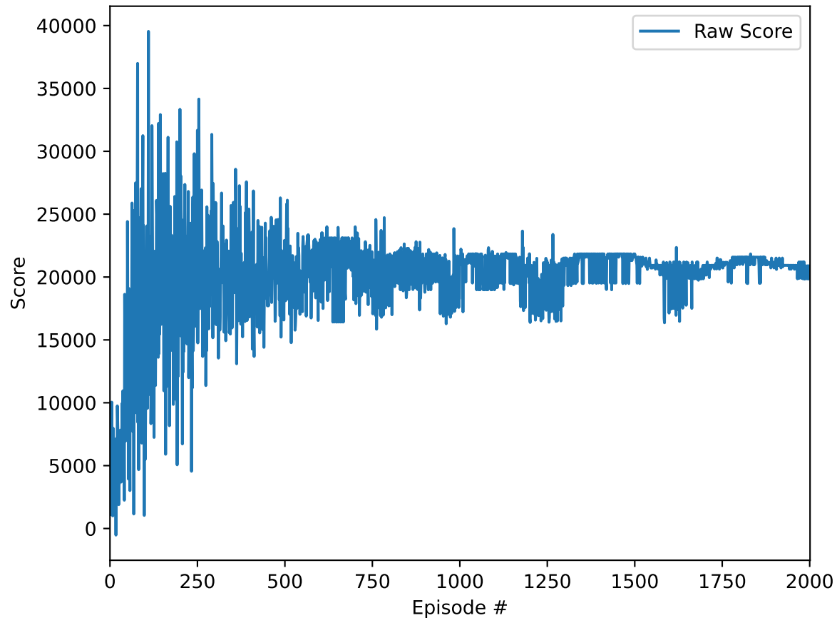
raw scores
