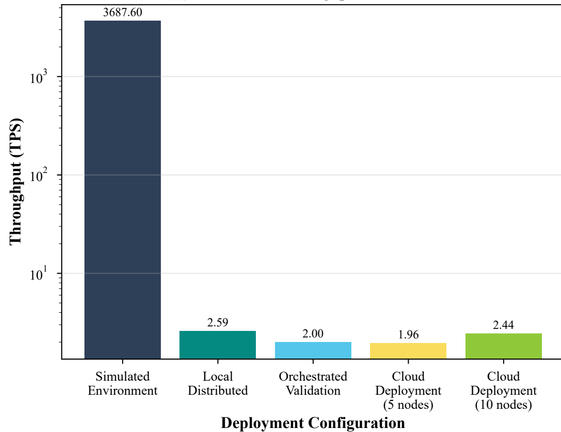
(a) Transaction Throughput Performance
