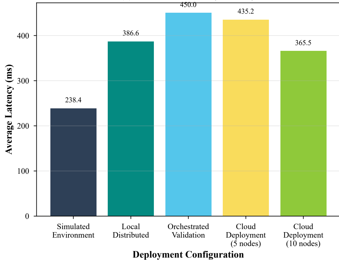
(b) Transaction Finality Latency
