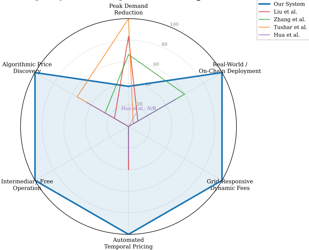
Capability Comparison Across Systems (Axis 1 is quantitative; axes 2-6 are author-assigned capability scores -- see figure note / SCORING_NOTES)
