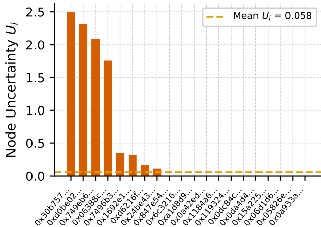
Node-Level Uncertainty per Entity
