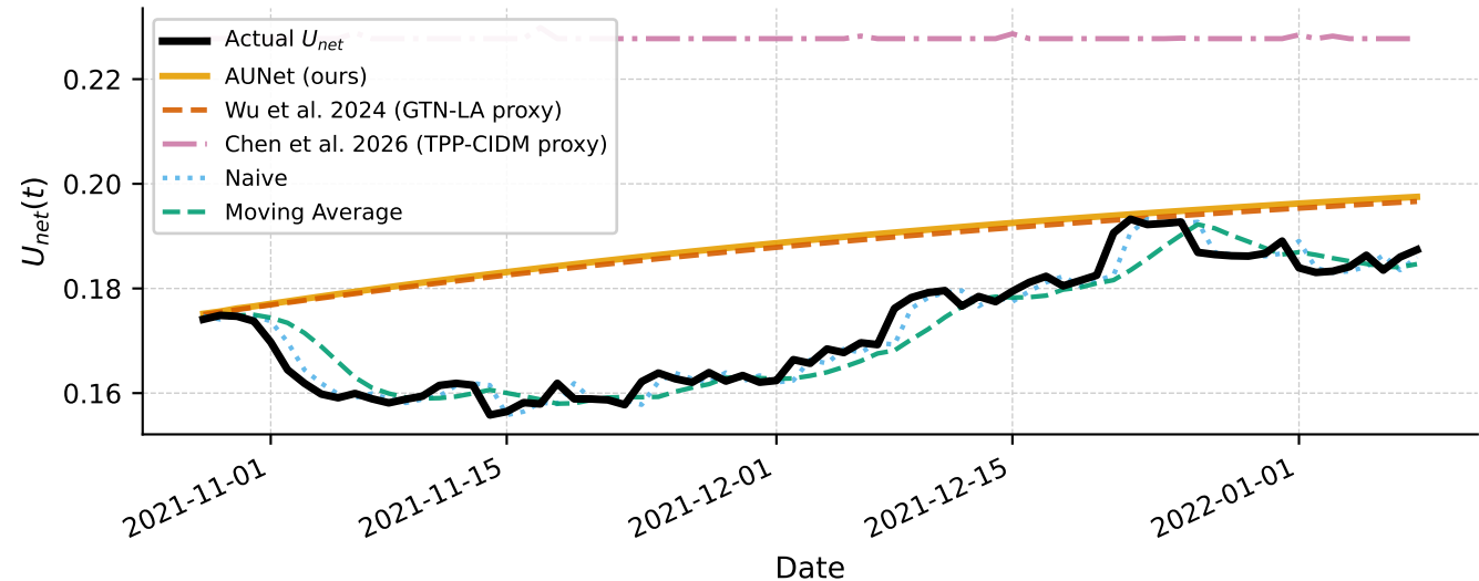
AUNet vs Baseline Methods — Test Window Prediction
