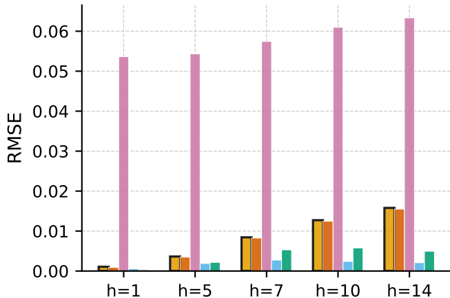
Prediction RMSE by Horizon
