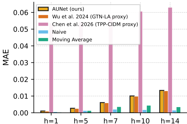
Prediction MAE by Horizon
