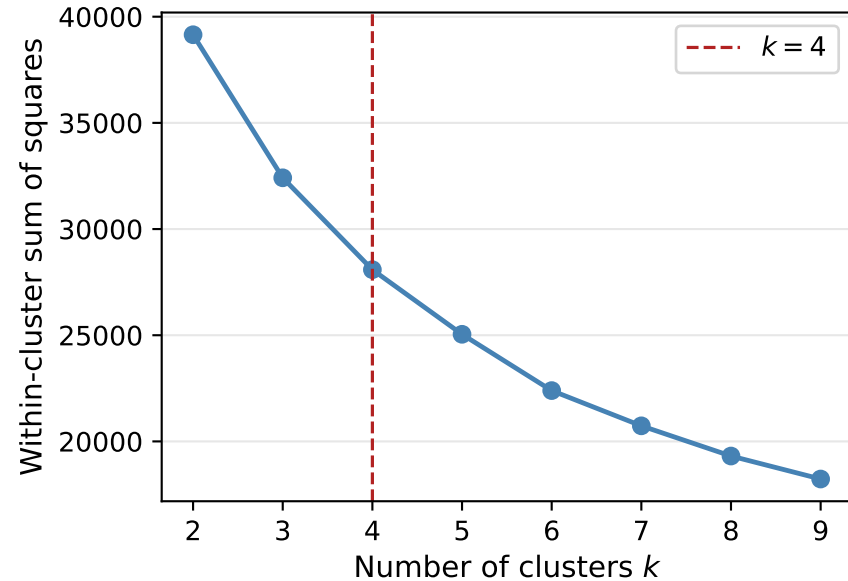
Elbow
