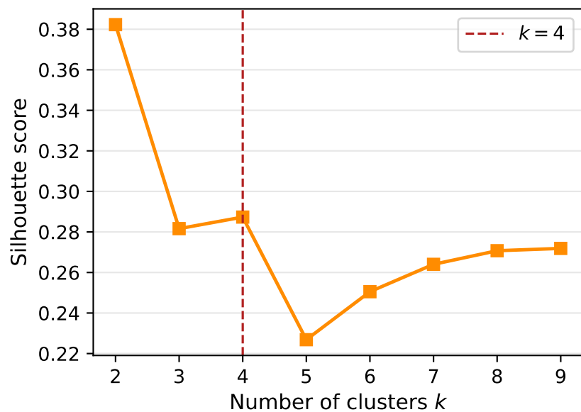
Silhouette
