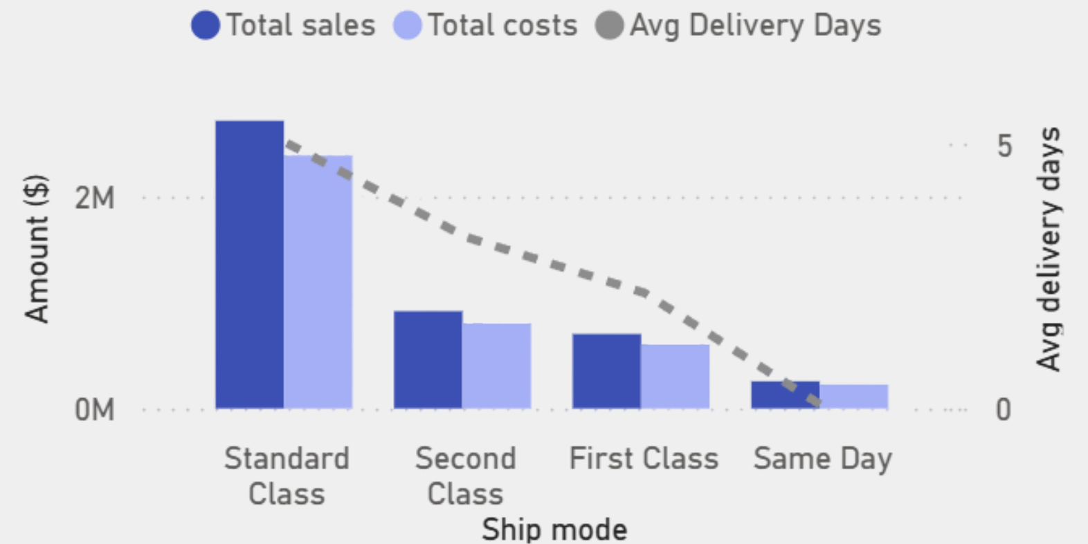
Sales, Costs & delivery days per ship mode
