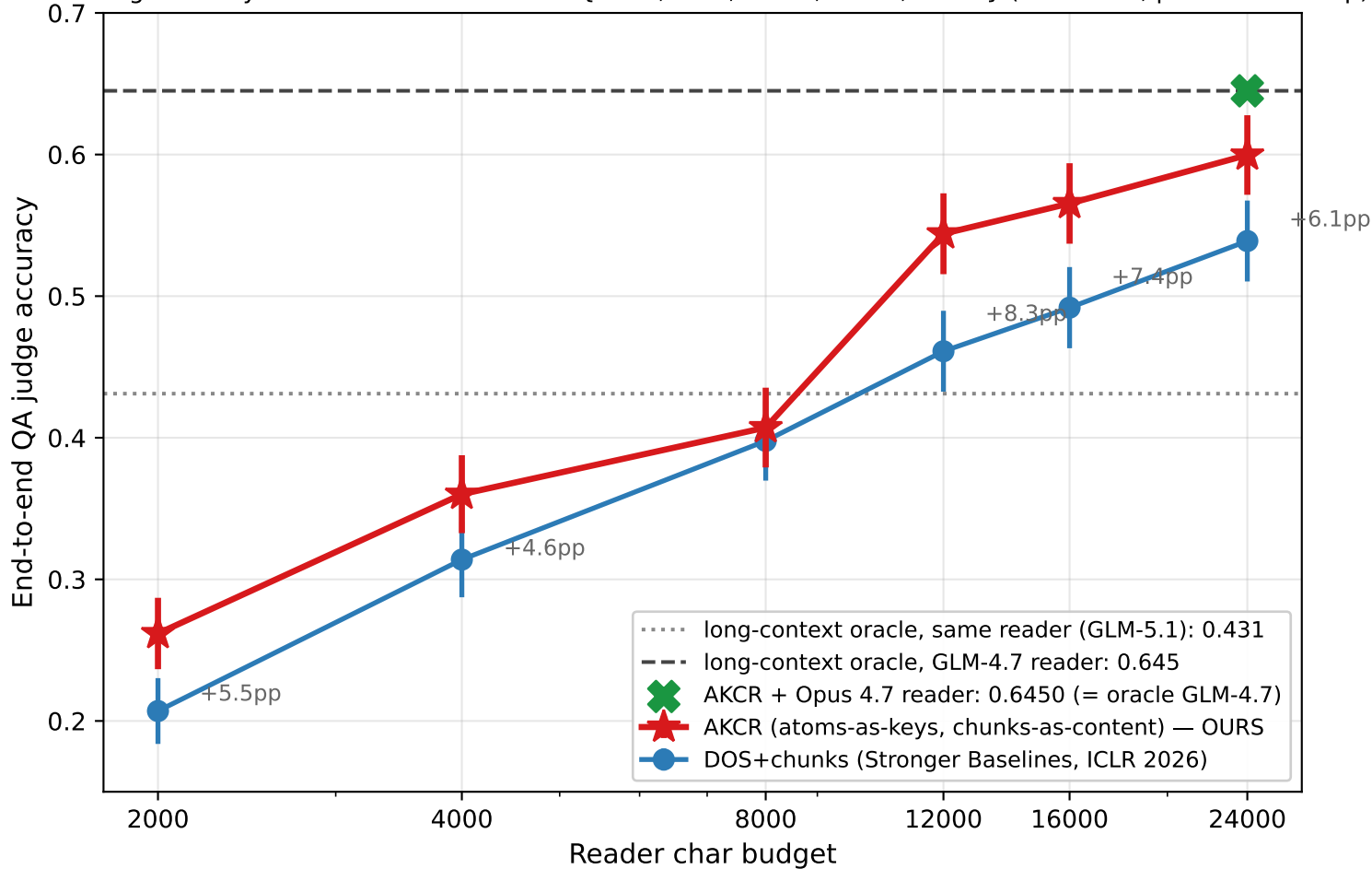
AKCR Pareto frontier (Full-book NarrativeQA, n=1169, GLM-5.1 reader)
