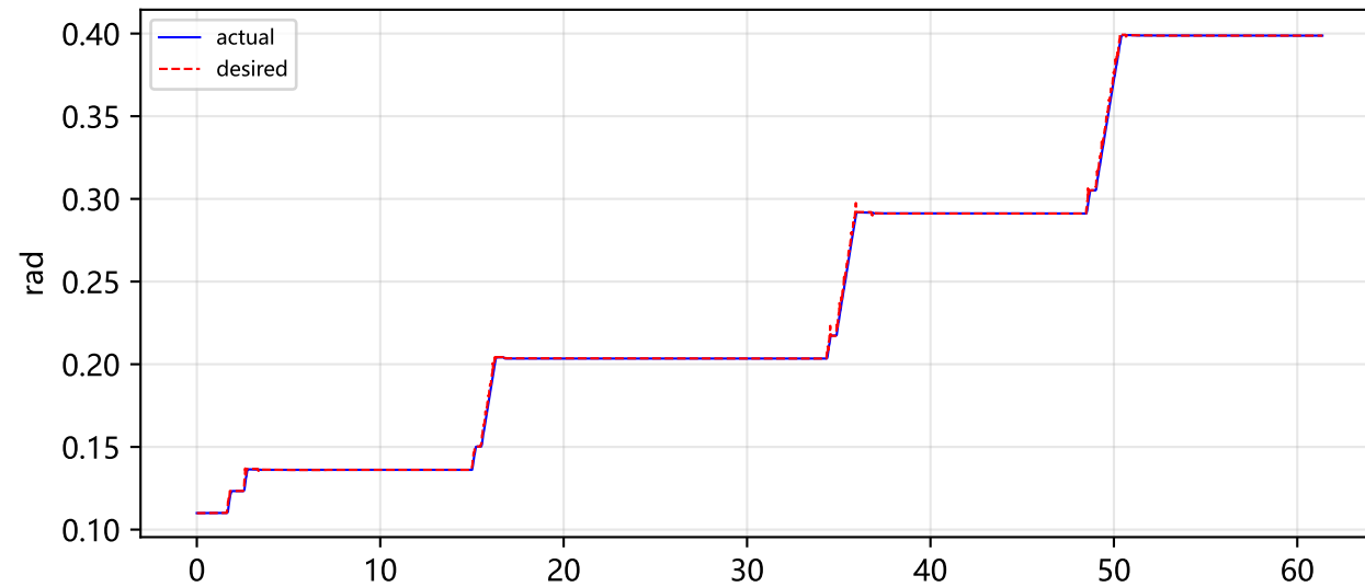
right_shoulder_yaw_joint
