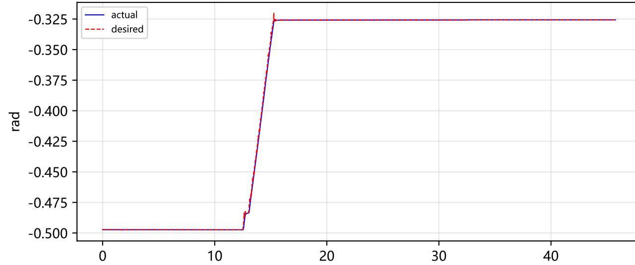
right_wrist_pitch_joint
