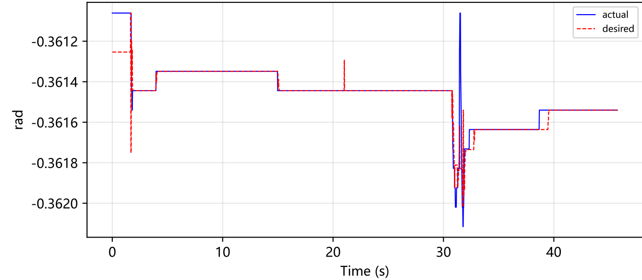
right_wrist_yaw_joint
