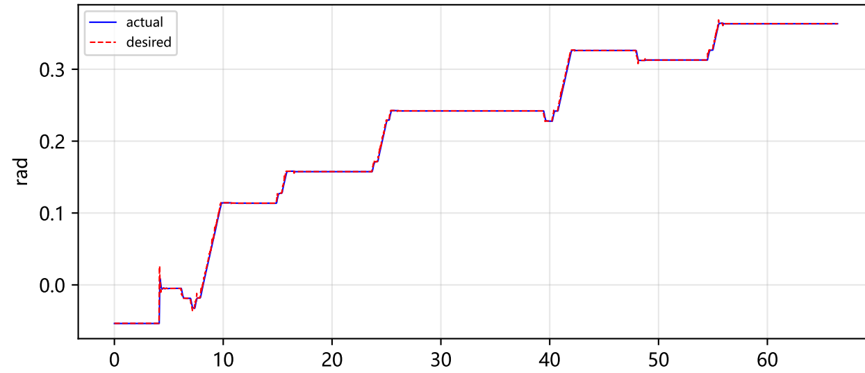
right_shoulder_yaw_joint
