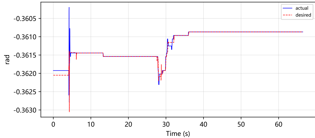
right_wrist_yaw_joint
