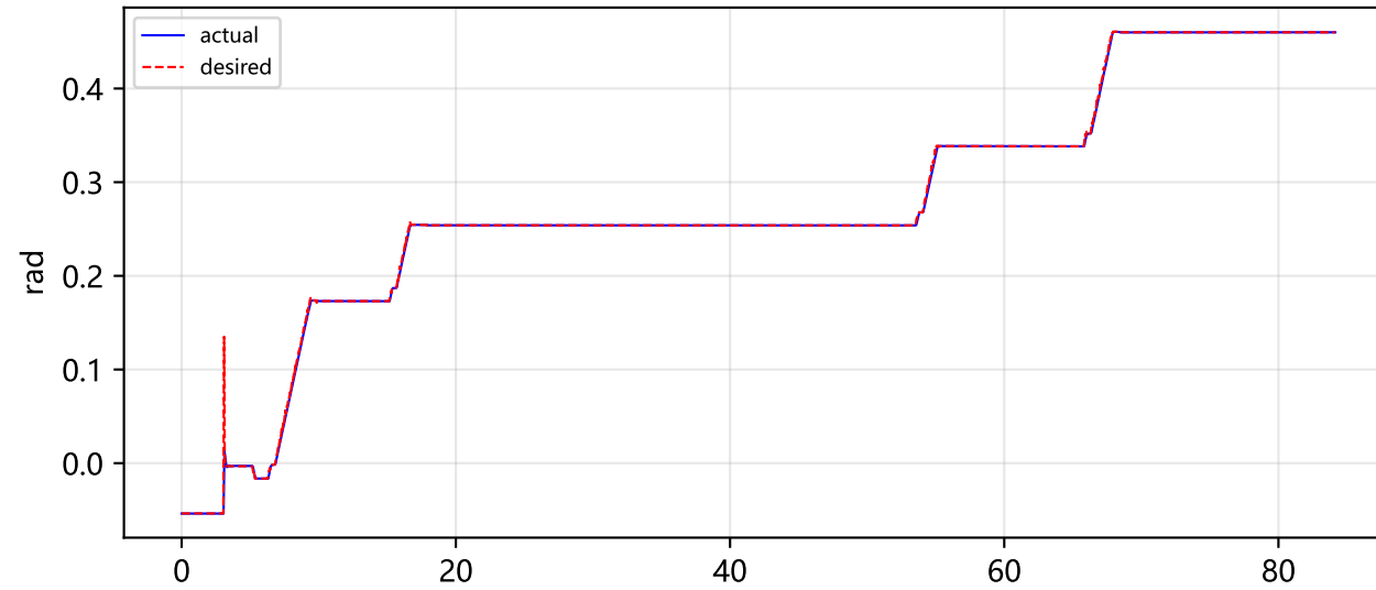
right_shoulder_yaw_joint
