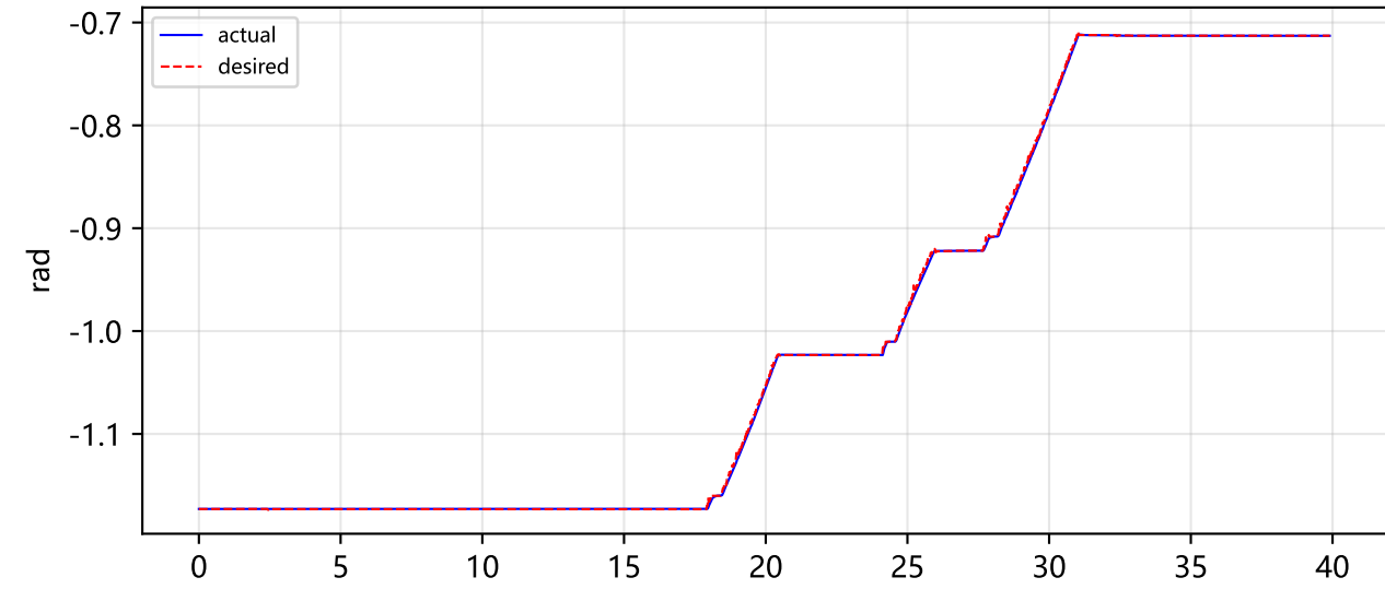
right_wrist_yaw_joint
