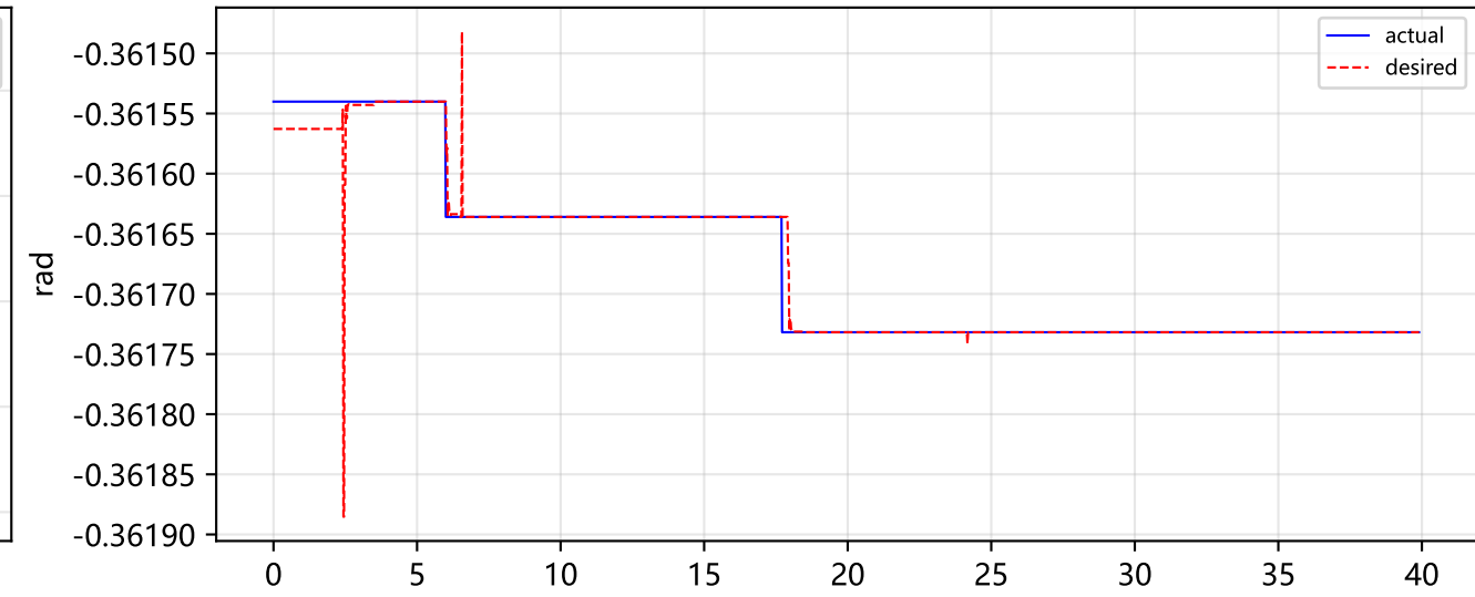
right_wrist_yaw_joint
