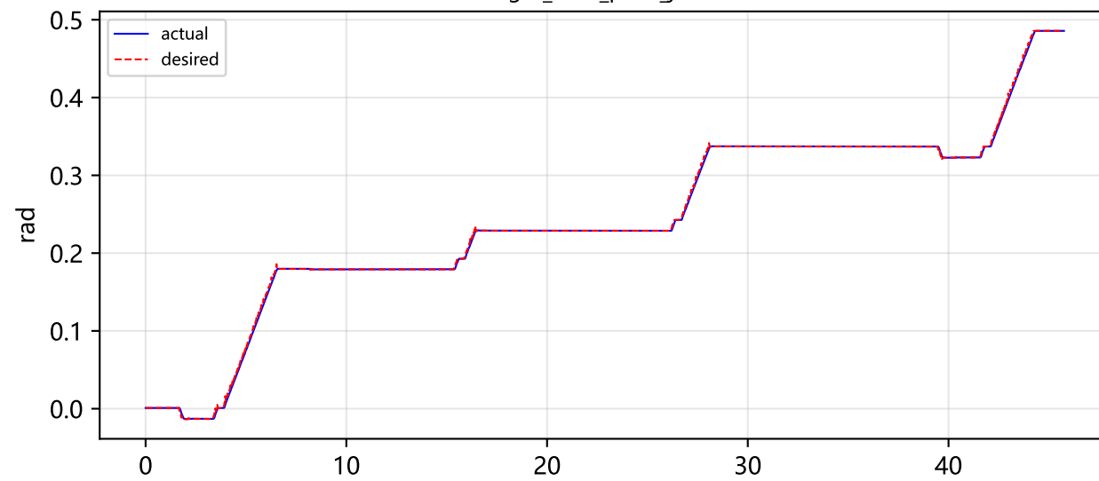
right_shoulder_yaw_joint
