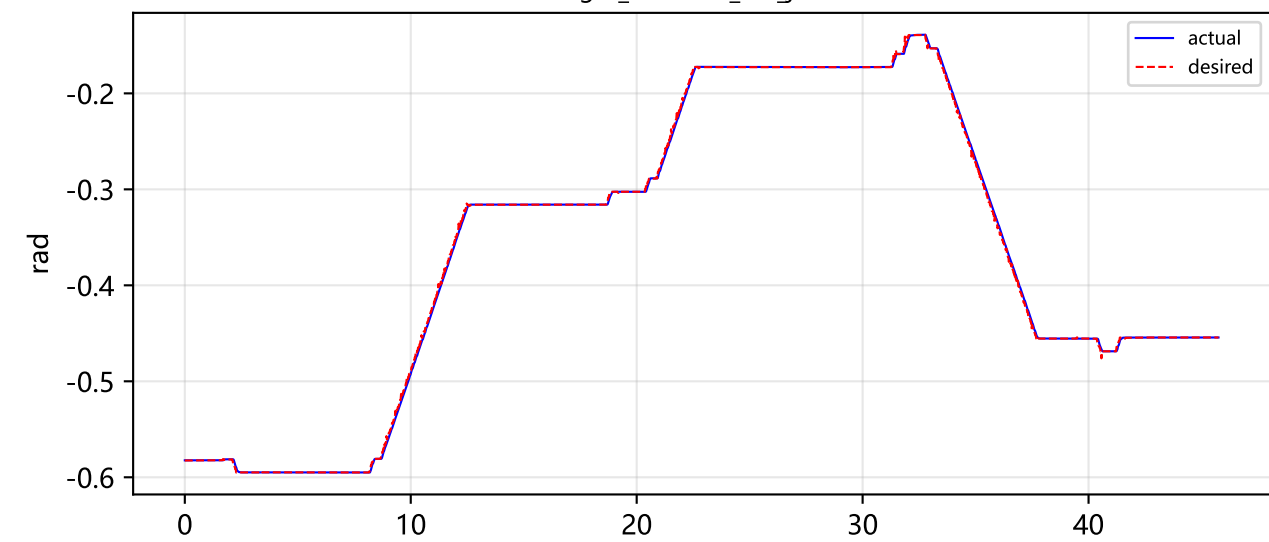
right_elbow_pitch_joint
