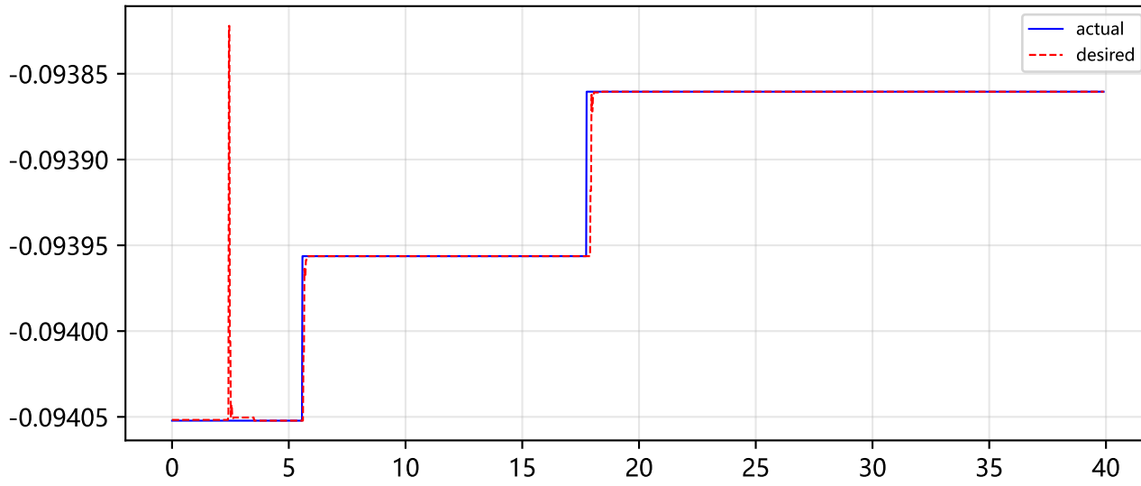
right_wrist_pitch_joint
