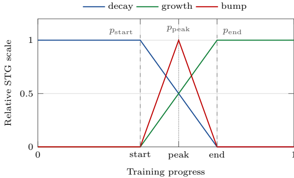
Figure 2: STG schedule shapes. Bump keeps late training free of structural amplification, avoiding per-view freezing on creative edits. The plot illustrates the three shapes; our method adopts the bump , with its peak placed around mid-training.
