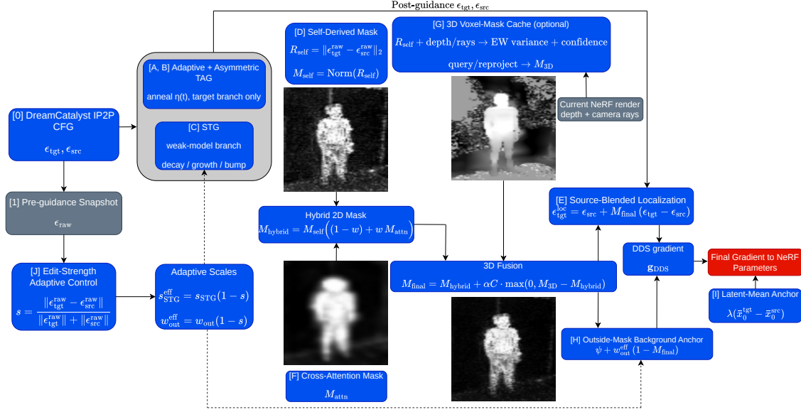
Figure 1: Method overview. DreamCatalyst’s IP2P CFG is extended with modular guidance, localization, and preservation branches: STG, adaptive/asymmetric TAG, self-derived masking, cross-attention masking, 3D voxel-mask aggregation, source-blended localization, outside-mask anchoring, latent-mean anchoring, and adaptive preservation controls. Defaults reproduce DreamCatalyst when these components are disabled.
