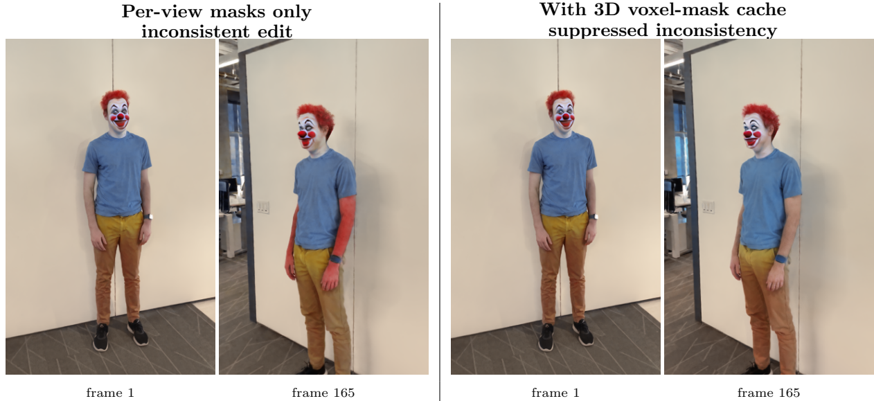
Figure 4: Qualitative motivation for the 3D voxel-mask cache. Without a 3D mask prior, the clown edit can become view-dependent: one training view accumulates arm/costume edits that another view does not. The voxel cache lifts high-confidence 2D mask evidence into world space and reprojects it to later views, suppressing this cross-view disagreement. A completed n=3 evaluation confirms that this benefit is qualitative: the cache makes residual failures view-coherent, while the aggregate image metrics stay within run-to-run noise.
