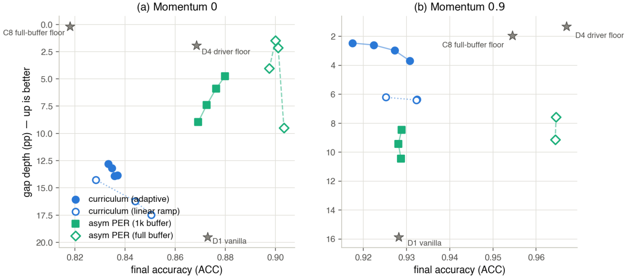
Figure C.2: Accuracy–depth scatter of every rot-MNIST gate condition: final accuracy (right is better) against gap depth (up is better, axis inverted). The \lambda -path (blue) is the curriculum, adaptive+ \lambda_{\min} as filled circles and linear ramps as open circles; the \delta -path (aqua) is asymmetric PER, the 1k buffer as filled squares and the full buffer as open diamonds, each sweeping \delta = 1.0 \rightarrow 0.03 ; grey stars are the anchors (no-gate D1, driver floor D4, full-buffer floor C8). (a) Momentum 0: at a matched 1k buffer the \delta -path dominates the \lambda -path, lower depth and higher accuracy, reaching the D4 floor. (b) Momentum 0.9: the apparent trade in this panel is a buffer mismatch: the directional gate’s high-accuracy points ( \approx 0.965 ) are its full 60k-buffer (open-diamond) legs, set against the curriculum’s practical 1k buffer. Held at a common buffer the panel collapses to the regime dependence of Section 6.4: momentum re-inflates the directional gate and the scalar gate becomes the lower-gap method.
