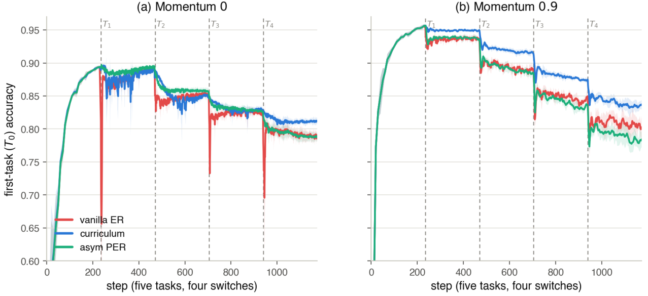
Figure C.3: Five-task rot-MNIST (rotations [0, 30, 60, 90, 120]^\circ , four consecutive switches, five seeds with \pm std bands), the refactored L-series: first-task T_0 accuracy across the whole sequence for vanilla ER (red), the shipping curriculum \lambda_{\min}=0.20 (blue) and asymmetric PER \delta=0.1 (aqua); dashed lines mark the four switches, and the two panels are the two momentum settings. (a) Momentum 0: both gates hold T_0 almost flat through every boundary — asymmetric PER the smoothest of all, with only shallow dips (smallest per-boundary area, Table C.10) — while vanilla ER takes a sharp instantaneous drop at each switch. This is the near-gap-free directional-gate regime the two-task sweep also finds at momentum 0. (b) Momentum 0.9: momentum re-inflates PER’s per-step filter, exactly as on the two-task benchmark (Section 6.3), so its boundary transients return and it tracks vanilla on cumulative retention; the curriculum keeps the boundaries smoothest and holds the highest plateau, the least cumulative forgetting on the long horizon. The single-transition reading thus carries past one boundary, and the momentum roles carry with it.
