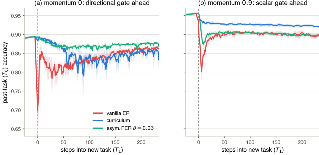
Figure 6.4: The momentum synthesis at the matched 1k buffer: per-step past-task ( T_0 ) accuracy across the rot-MNIST switch for vanilla ER (red), the shipping curriculum C7 (blue), and asymmetric PER at its strongest standard-buffer filter \delta=0.03 (aqua); seed mean with \pm std bands, x=0 the task switch. (a) Momentum 0: the directional gate holds T_0 highest (4.8 pp / ACC 0.880) while the curriculum opens a deep, noisy dip (13.9 pp / 0.837). (b) Momentum 0.9: the ordering swaps: the curriculum holds T_0 near its plateau (3.7 pp / 0.931) while accumulated velocity re-inflates the directional gate’s per-step filter (8.5 pp / 0.929). The pre-switch level is higher in (b) because momentum converges T_0 higher before the switch.
