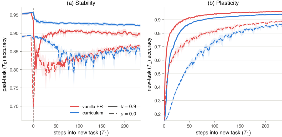
Figure 6.2: The scalar feedback gate and momentum’s two roles: per-step accuracy across the rot-MNIST switch, seed mean with \pm std bands, for vanilla ER (red) and the shipping adaptive curriculum \lambda_{\min}=0.20 (blue), each at momentum 0.9 (solid) and 0.0 (dashed). (a) Stability ( T_0 ): only curriculum-with-momentum (solid blue) holds the past task near its plateau through the switch; momentum barely dents vanilla’s spike (solid red still dives), and both methods open a deep, jittery gap without it (dashed). Momentum closes the gap where the gate has already tempered the push at source, not otherwise. (b) Plasticity ( T_1 ): at momentum 0 the curriculum slows early new-task learning (dashed blue is slowest to rise, the plasticity debt of holding the push down), but momentum pays it back, lifting the solid-blue curve back toward the vanilla pace.
