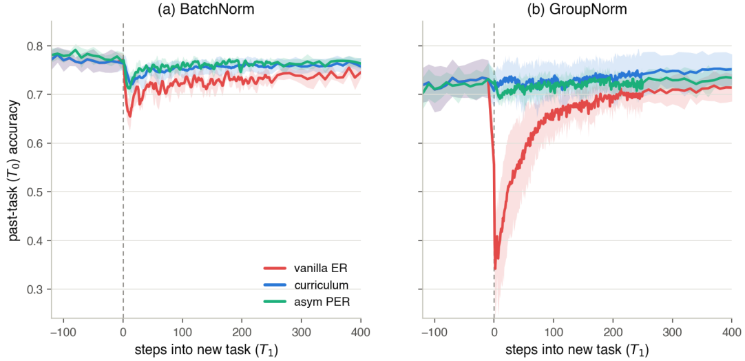
Figure 6.5: Per-step past-task ( T_0 ) accuracy across the CIFAR-10 transition (ResNet-18, momentum 0.9, buffer 5,000), one panel per normalisation, each overlaying vanilla ER (red), the shipping curriculum (blue) and asymmetric PER (aqua); seed mean with \pm std bands, x=0 the task switch. (a) BatchNorm: vanilla ER dips and re-adapts slowly while both gates hold T_0 near its plateau. (b) GroupNorm: vanilla ER crashes T_0 almost to chance and crawls back over the whole recovery window, whereas both gates hold it flat through the switch, cutting the deep transient and lifting worst-case retention from \approx 0.31 to \approx 0.67 . On this backbone the transient stays open for hundreds of steps, so the area carries as much of the comparison as the depth (Table 6.3, Appendix C.5).
