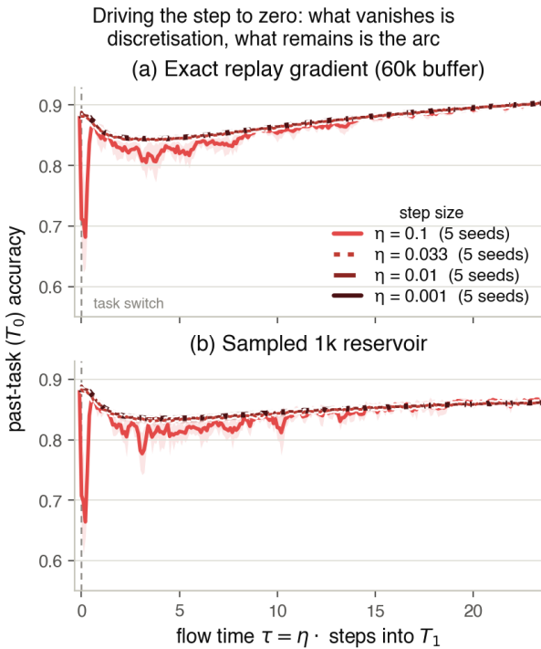
Figure 6.1: The effect of step size ( \eta ) on past-task accuracy during a task switch. Across both (a) exact gradients and (b) standard reservoir replay, reducing the step size eliminates the sharp initial boundary spike caused by the standard learning rate ( \eta = 0.1 ). Crucially, a smooth performance dip (the “arc”) remains across all finer step sizes, demonstrating that this underlying drop is a fundamental property of the trajectory, rather than an optimization artifact.
