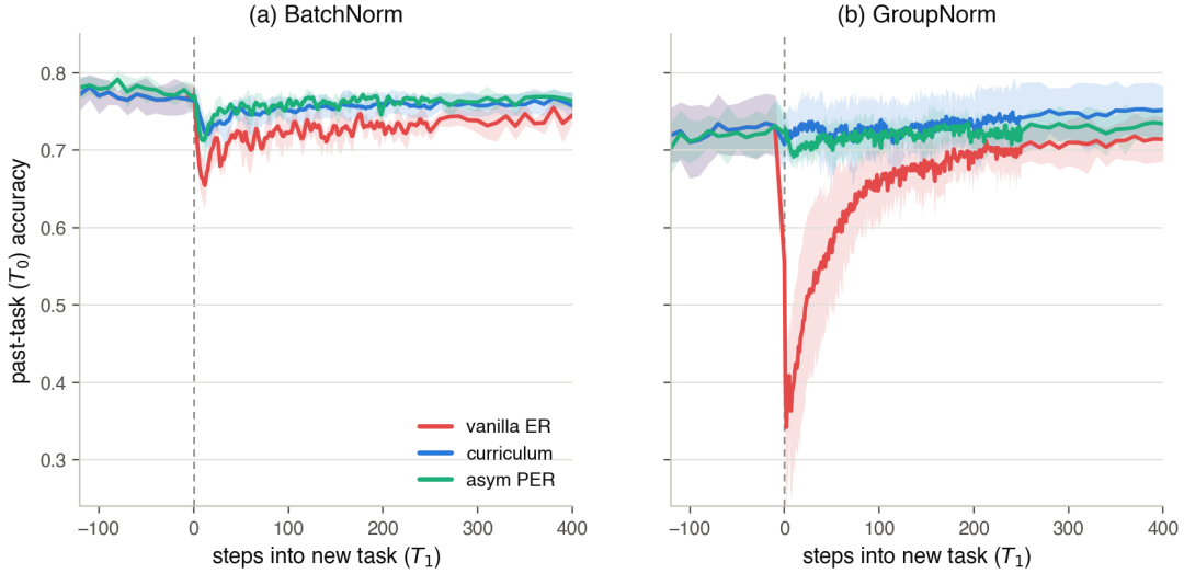
Figure 6.5: Per-step past-task ( T_0 ) accuracy across the CIFAR-10 transition (ResNet-18, momentum 0.9, buffer 5,000), one panel per normalisation, each overlaying vanilla ER (red), the practical curriculum (blue) and asymmetric PER (aqua); seed mean with \pm std bands, x=0 the task switch. (a) BatchNorm: vanilla ER dips and re-adapts slowly while both gates hold T_0 near its plateau. (b) GroupNorm: vanilla ER’s transient is deep and long, whereas both gates hold T_0 flat through the switch (Table 6.3, Appendix C.6).
