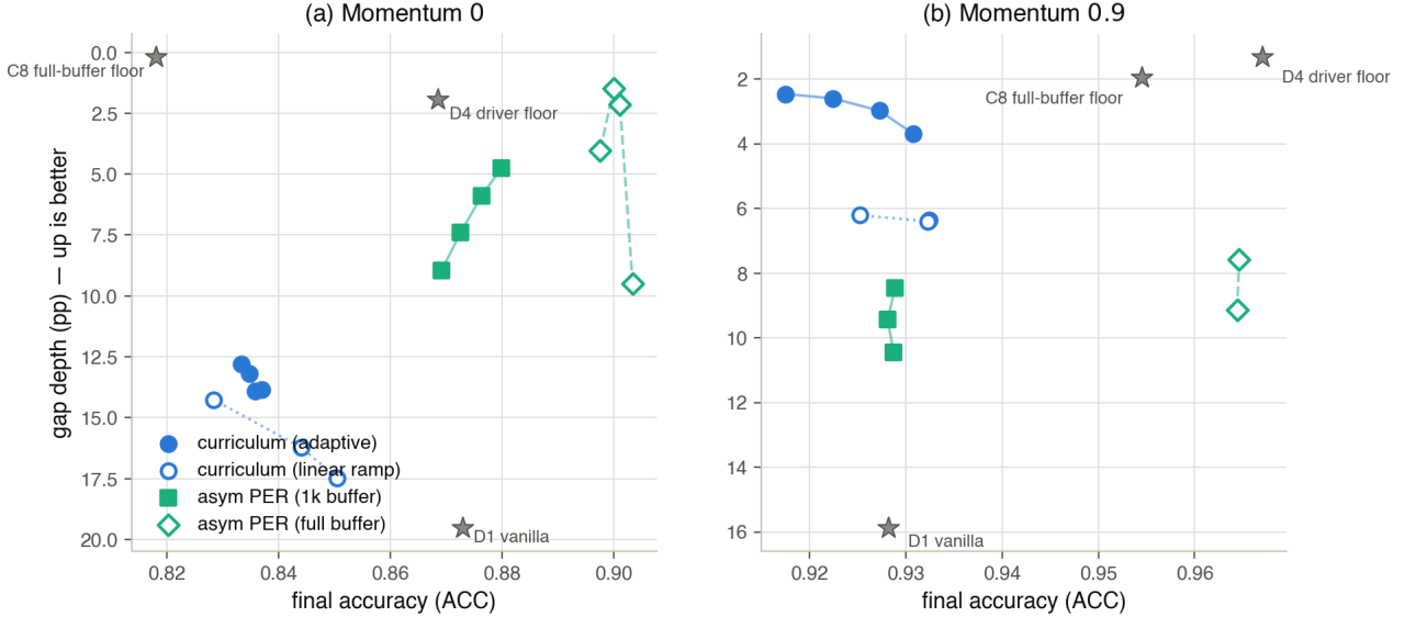
Figure C.1: Accuracy–depth scatter of every rot-MNIST gate condition: final accuracy (right is better) against gap depth (up is better, axis inverted). The \lambda -path (blue) is the curriculum, adaptive+ \lambda_{\min} as filled circles and linear ramps as open circles; the \delta -path (aqua) is asymmetric PER, the 1k buffer as filled squares and the full buffer as open diamonds, each sweeping \delta = 1.0 \rightarrow 0.03 ; grey stars are the anchors (no-gate D1, driver floor D4, full-buffer floor C8). (a) Momentum 0: at a matched 1k buffer the \delta -path dominates the \lambda -path, lower depth and higher accuracy, reaching the D4 floor. (b) Momentum 0.9: the apparent trade in this panel is a buffer mismatch — the directional gate’s high-accuracy points ( \approx 0.965 ) are its full 60k-buffer (open-diamond) legs, set against the curriculum’s practical 1k buffer. Held at a common buffer the panel collapses to the regime flip of Section 6.4: momentum re-inflates the directional gate and the scalar gate becomes the lower-gap method. This figure is retained as the underlying scatter; the frontier reading it once suggested is superseded.
