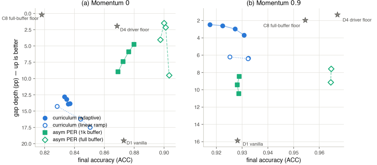
Figure C.2: Accuracy–depth scatter of every rot-MNIST gate condition: final accuracy (right is better) against gap depth (up is better, axis inverted). The \lambda -path (blue) is the curriculum, adaptive+ \lambda_{\min} as filled circles and linear ramps as open circles; the \delta -path (aqua) is asymmetric PER, the 1k buffer as filled squares and the full buffer as open diamonds, each sweeping \delta = 1.0 \rightarrow 0.03 ; grey stars are the anchors (no-gate D1, driver floor D4, full-buffer floor C8). (a) Momentum 0: at a matched 1k buffer the \delta -path dominates the \lambda -path, lower depth and higher accuracy, reaching the D4 floor. (b) Momentum 0.9: the apparent trade in this panel is a buffer mismatch: the directional gate’s high-accuracy points ( \approx 0.965 ) are its full 60k-buffer (open-diamond) legs, set against the curriculum’s practical 1k buffer. Held at a common buffer the panel collapses to the regime dependence of Section 6.4: momentum re-inflates the directional gate and the scalar gate becomes the lower-gap method.
