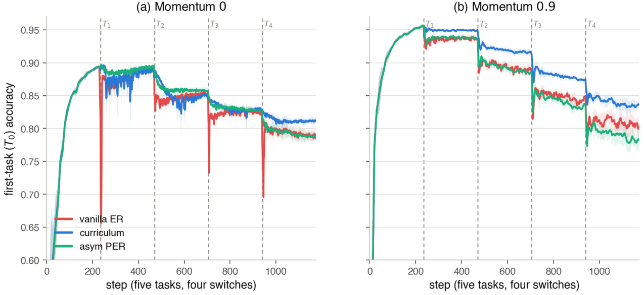
Figure C.3: Five-task rot-MNIST (rotations [0, 30, 60, 90, 120]^\circ , four consecutive switches, five seeds with \pm \text{std} bands), the L-series: first-task T_0 accuracy across the whole sequence for vanilla ER (red), the practical curriculum \lambda_{\min}=0.20 (blue) and asymmetric PER \delta=0.1 (aqua); dashed lines mark the four switches, and the two panels are the two momentum settings. (a) Momentum 0: both gates hold T_0 almost flat through every boundary — asymmetric PER the smoothest of all, with only shallow dips (smallest per-boundary area, Table C.11) — while vanilla ER takes a sharp instantaneous drop at each switch. This is the near-gap-free directional-gate regime the two-task sweep also finds at momentum 0. (b) Momentum 0.9: momentum re-inflates PER’s per-step filter, exactly as on the two-task benchmark (Section 6.3), so its boundary transients return and it tracks vanilla on cumulative retention; the curriculum keeps the boundaries smoothest and holds the highest plateau, the least cumulative forgetting on the long horizon. The single-transition reading thus carries past one boundary, and the momentum roles carry with it.
