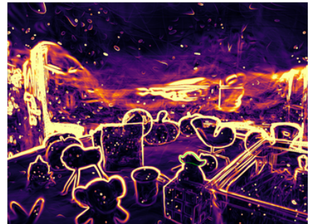
Figure 4. Selected alpha/depth discontinuity boundary cases for the strict pad16 SAM3-box direct-3D readout. Cases are selected from Table 12’s worst boundary-error records, with scene coverage enforced before filling remaining slots. The overlays show that high discontinuity often co-occurs with failure cases, but the weak query-level correlations keep this figure as mechanism context rather than a causal proof.
