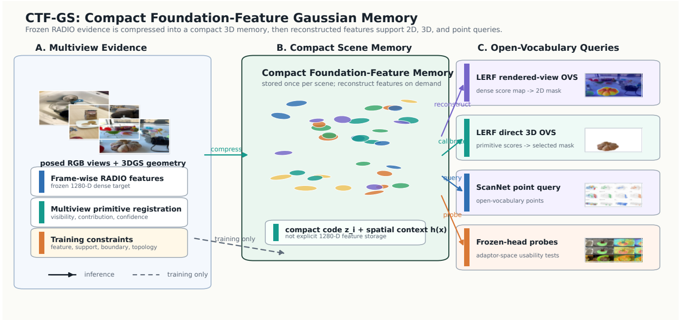
Fig. 1. CTF-GS framework. A pretrained 3DGS scene supplies geometry, while frozen RADIO supplies the dense foundation feature to be reconstructed. The method stores compact per-Gaussian latent codes with spatial context and quality/visibility cues, then reconstructs RADIO-compatible scene features by global decoders. SigLIP2, DINOv3, and SAM3 adaptor spaces are used as frozen-head constraints or probes of the reconstructed RADIO feature, not as separate raw feature memories. Multiview Primitive Registration compresses registered semantic evidence into the same compact memory during training. At inference, the memory supports rendered 2D query, direct Gaussian selection, and point-level query without a multiview-registration feature cache or official RGB SAM decoder.
