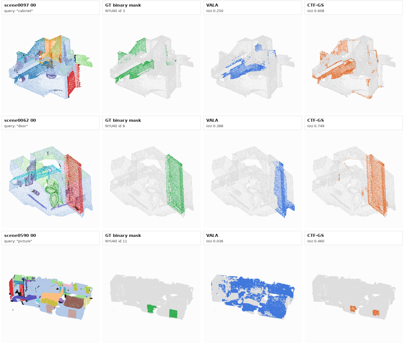
Fig. 4. ScanNet open-vocabulary 3D query qualitative comparison. Each row shows a binary text-class query on a VALA/OpenGaff-8 scene: scene overview, GT class points, our local VALA compatibility reproduction, and CTF-GS direct point-query prediction. Gray points are non-query classes.
