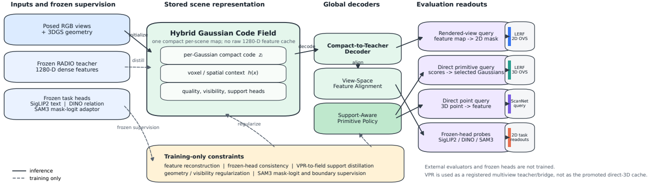
Figure 1. CTF-GS framework. The method stores one compact foundation-feature Gaussian map with per-Gaussian codes, spatial context, and quality/visibility heads, then decodes it into teacher-compatible features. The same map supports three inference readouts: rendered dense feature maps for LERF 2D open-vocabulary grounding, compact primitive scores with a support-aware policy for LERF direct 3D object selection, and direct point features for ScanNet queries. Frozen RADIO/SigLIP2/DINOv3/SAM3 heads, VPR-to-field support distillation, and geometry/visibility losses are used only as training constraints; VPR is a registered multiview teacher/bridge rather than the promoted direct-3D cache.
