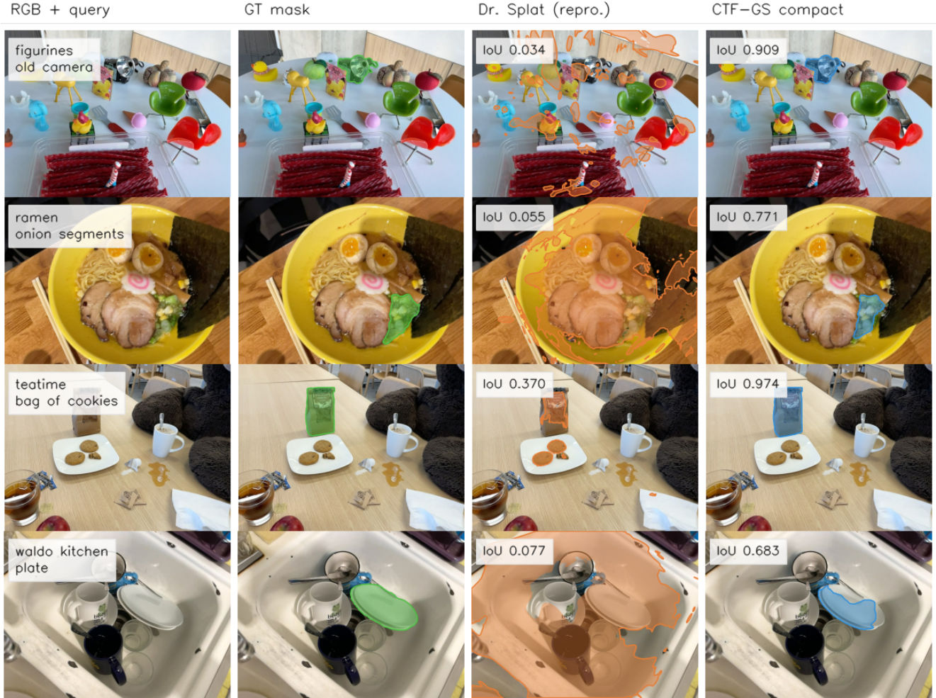
Figure 2. Main LERF qualitative comparison under the direct-3D object-selection protocol. Each row fixes a scene, annotated frame, and text query, then shows the RGB input, ground-truth mask, a reproduced Dr. Splat mask, and our compact direct-field mask. IoU is shown per panel for auditability. CTF-GS queries the compact foundation-feature Gaussian map directly; VPR is used only as a training teacher and no official RGB SAM3 boundary readout is used for these predictions.
