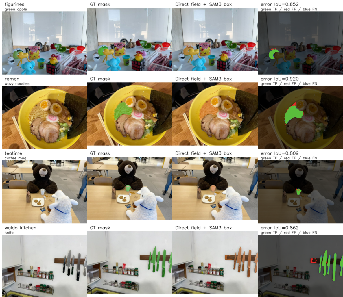
Fig. 3. Boundary-assisted direct-3D examples using the SAM3-box control. This variant illustrates a boundary readout after compact primitive selection and is separate from the strict compact one-map ablation.
