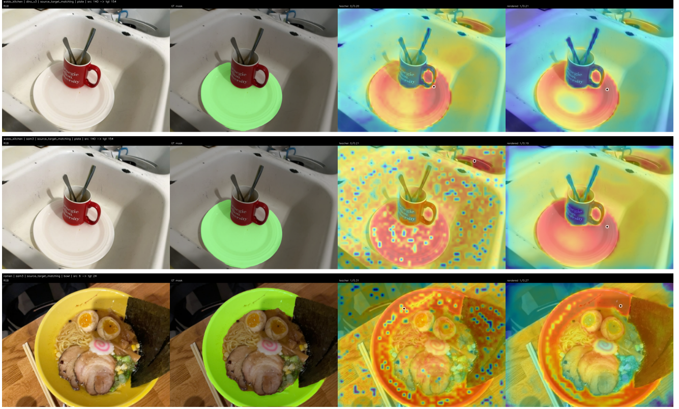
Figure 4. Qualitative DINOv3/SAM3 adaptor-space source-target matching. Each row shows RGB, GT mask, original RADIO teacher heatmap, and CTF-GS rendered heatmap. The Waldo Kitchen rows show cases where rendered features move the peak onto the target object; the Ramen row illustrates that the aggregate SAM3 gap remains visible even when localization is correct.
