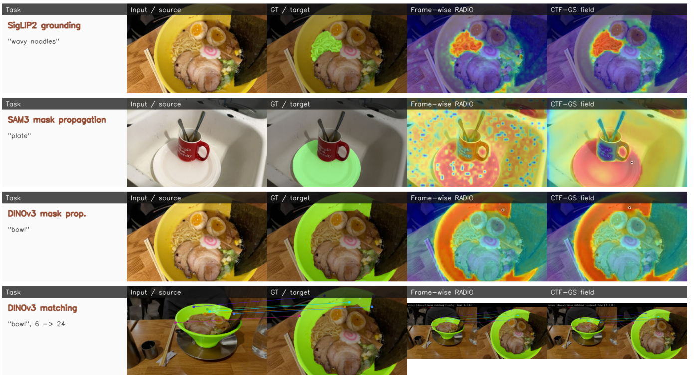
Fig. 7. Reconstructed scene features versus frame-wise RADIO under frozen-head tasks. Columns compare the task input/GT, frame-wise RADIO response, and GaussFM reconstructed field response for SigLIP2 grounding, SAM3-adaptor mask propagation, DINOv3 mask propagation, and DINOv3 dense matching.
