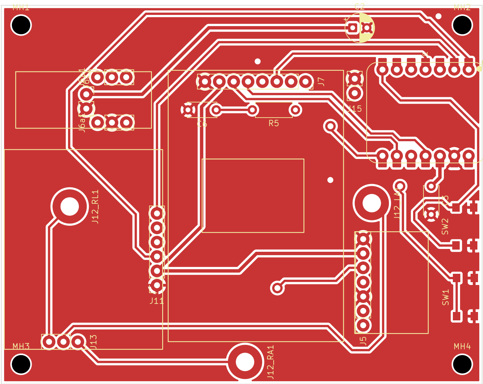
Supaclock v1 - Carrier 67x85mm
