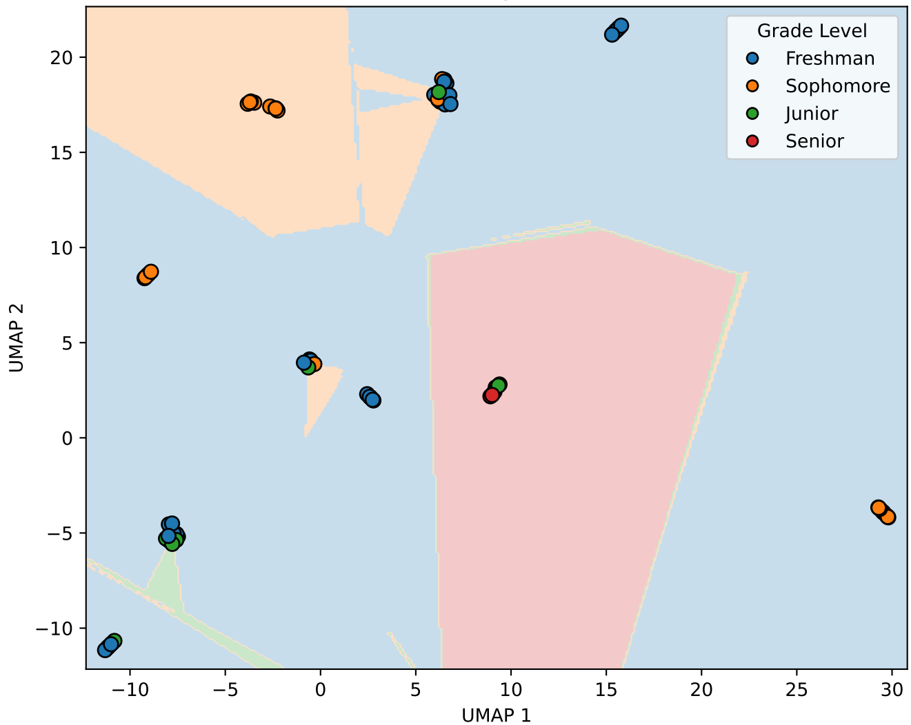
5-NN clusters on UMAP embedding (CV acc 0.6458781362007168)
