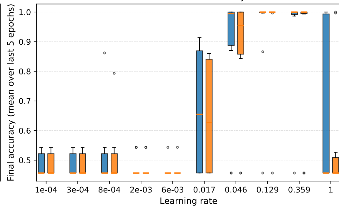
Unbalanced — Accuracy
