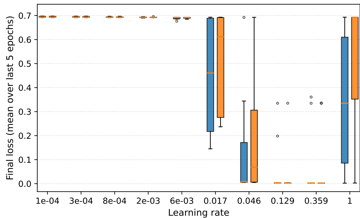
Unbalanced — Loss
