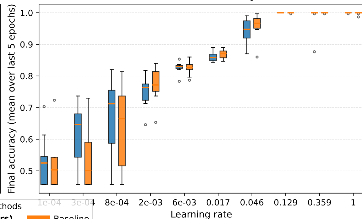
Unbalanced — Accuracy
