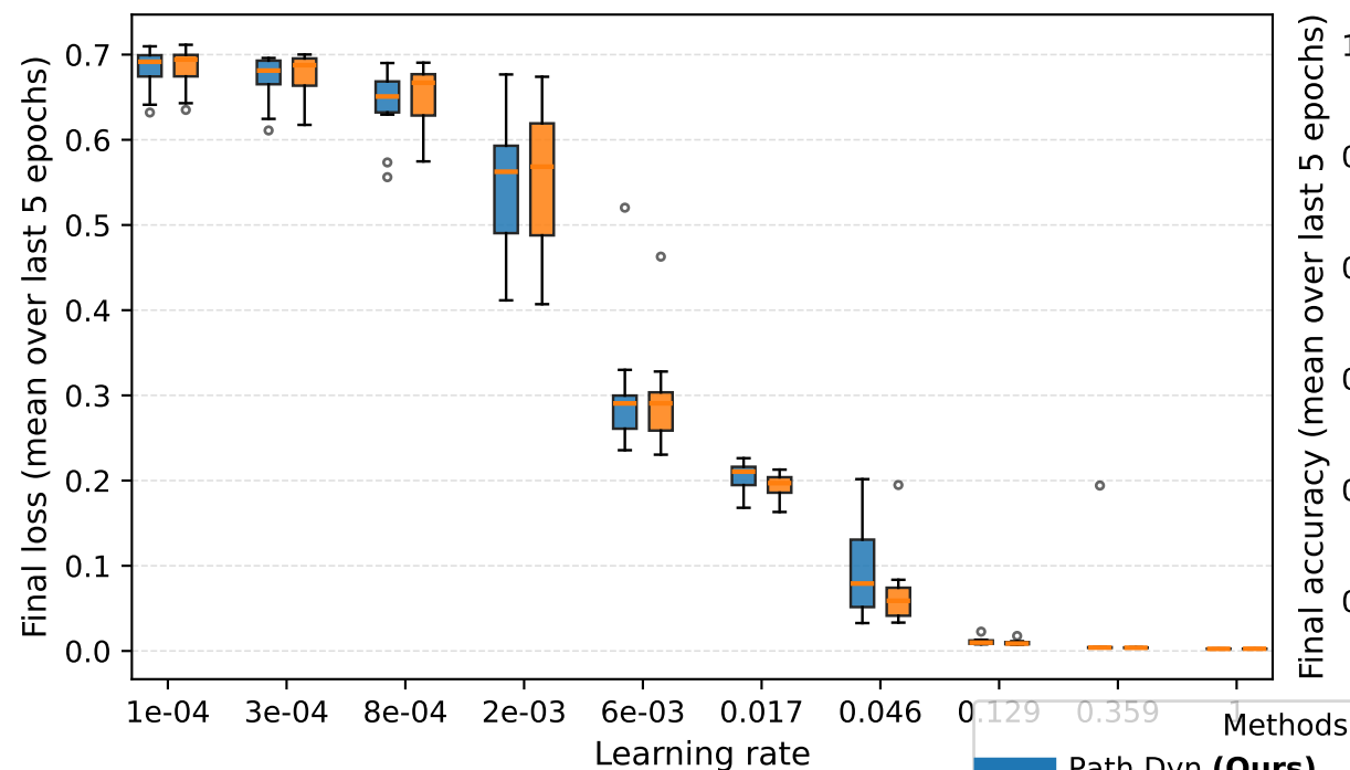
Unbalanced — Loss
