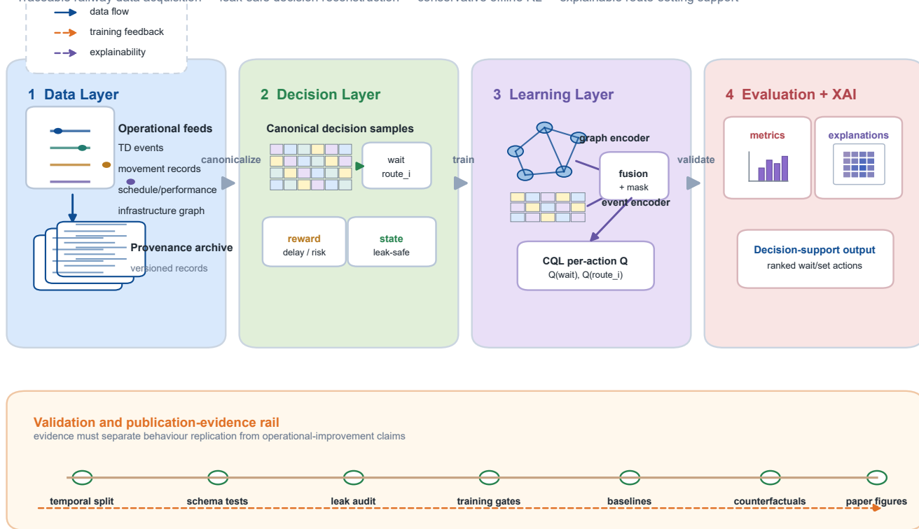
Figure 1. Reference-style system architecture of RailRL for railway route-setting decision support.
