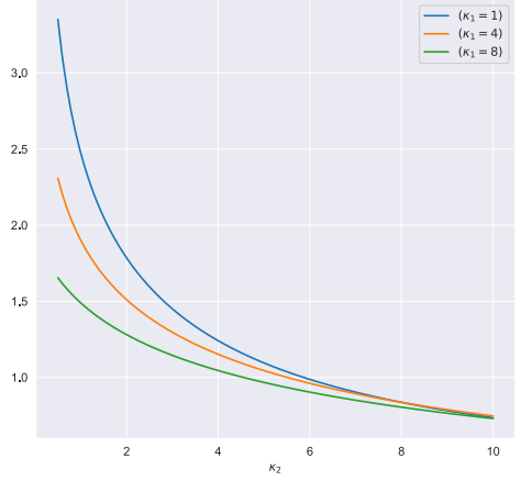
(b) Skewness of volatility as function of k_2
