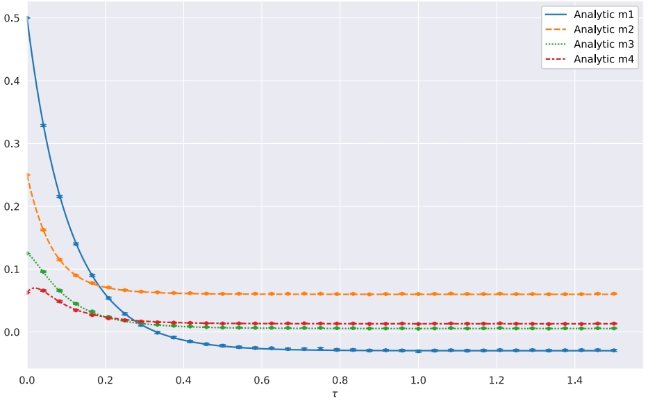
(b) Volatility of moments with k^* = 8
