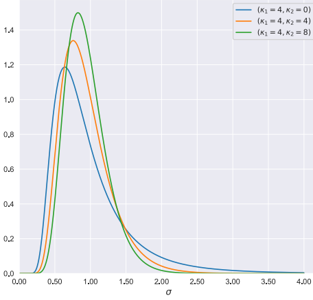
(a) Steady state distribution of the volatility
