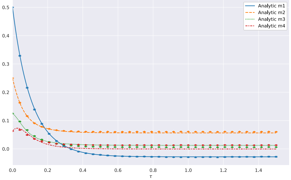
(a) Volatility of moments with k^* = 4
