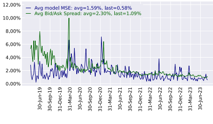
(a) Average mean-squared error and bid-ask volatility spread
