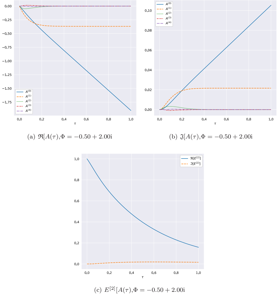
Fig. 5. The solution of ODEs in Eq. (4.25) as function of \tau for \Phi = -0.5 + 2i , p = 1 . We use the model parameters calibrated to Bitcoin options data and reported in Eq. (6.4). (a) The real part of the solution, (b) the imaginary part of the solution, (c) the real and imaginary parts of the exponential term E^{[2]} in Eq. (4.24).
