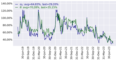
(c) Volatility beta
