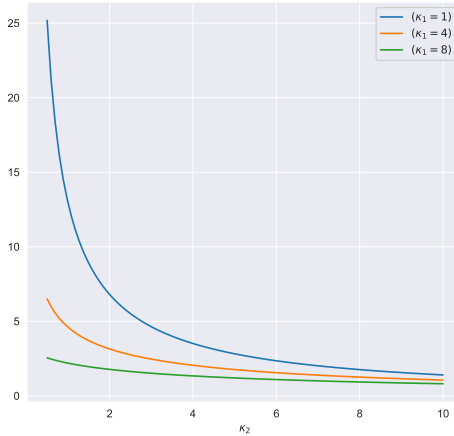
(c) Excess kurtosis of log-returns as function of k_2
