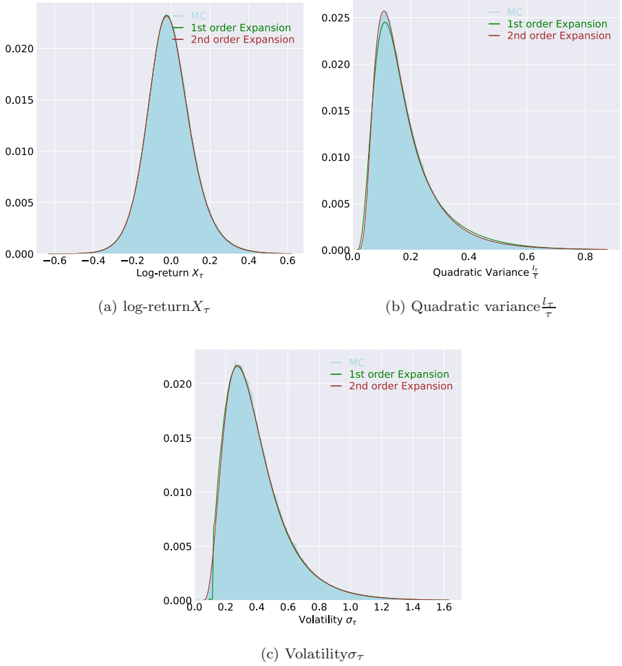
Fig. 6. PDFs computed using the inversion of the first order expansion term E^{[1]} in Eq. (4.16) and the second-order expansion term E^{[2]} in Eq. (4.24) for the state variables under the MMA measure: (a)–(c) PDFs of log-return, X_\tau , of QV normalized by \tau , I_\tau/\tau , of volatility \sigma_\tau , \sigma_\tau = Y_\tau + \theta , respectively. We use the model parameters for Bitcoin options reported in Eq. (6.4) with time to maturity of one month, \tau = 1.0/12.0 . The blue histogram is computed using realizations from MC simulations of joint model dynamics (3.12) using scheme in Eq. (3.59) with the number of path equal 400,000 and daily time steps.
