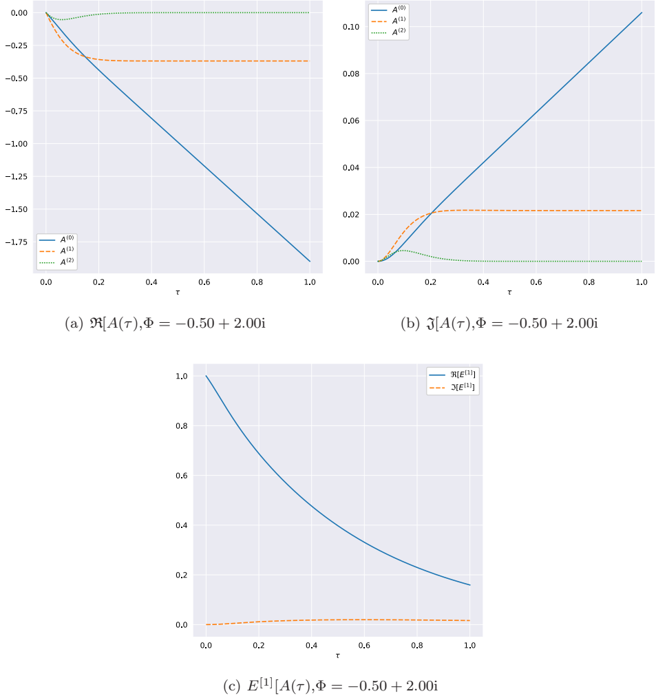
Fig. 4. The solution of ODEs of the first order expansion in Eq. (4.17) as function of \tau for \Phi = -0.5 + 2i , p = 1 . We use the model parameters calibrated to Bitcoin options data and reported in Eq. (6.4). (a) The real part of the solution, (b) the imaginary part of the solution, (c) the the real and imaginary parts of the exponential term E^{[1]} in Eq. (4.16).
