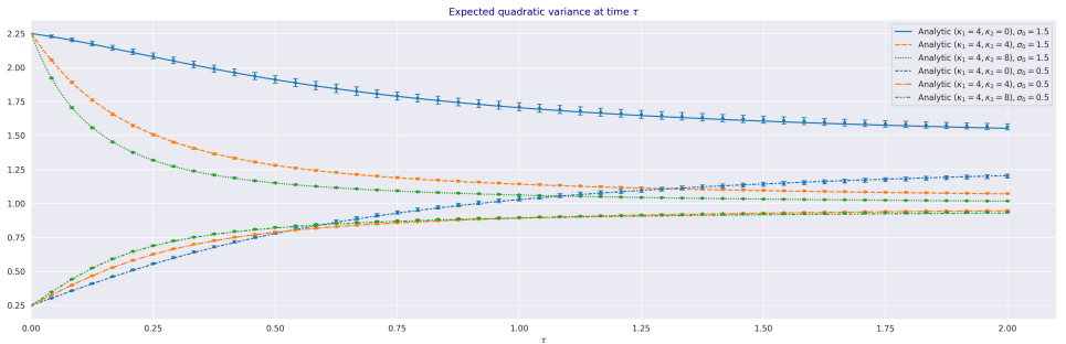
Fig. 3. The expected QV computed using Eq. (3.53) with k^* = 4 . The top and bottom three lines correspond to \sigma_0 = 1.5 and \sigma_0 = 0.5 , respectively. The dot and the error bars denote the estimate and 95% confidence interval computed using MC simulations of model dynamics with scheme in SDE (3.59) with number of path equal 100 000 and daily time steps. The model cases of mean-reversion correspond to \kappa_1 = 4 and three choices \kappa_2 = \{0, 4, 8\} with other model parameters set to \theta = 1.0 , \vartheta = 1.5 .
