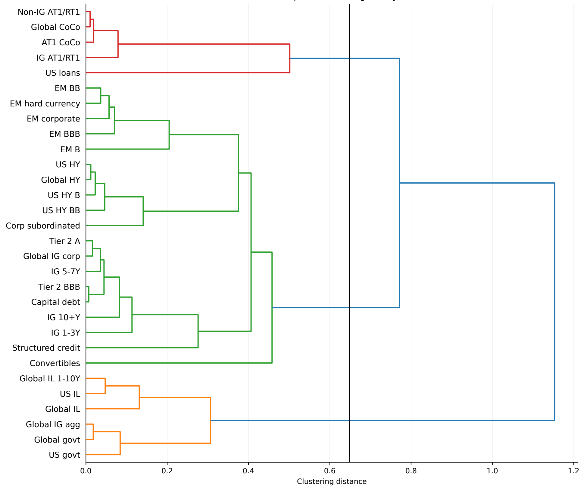
FactorLasso response clustering at 30 June 2026
