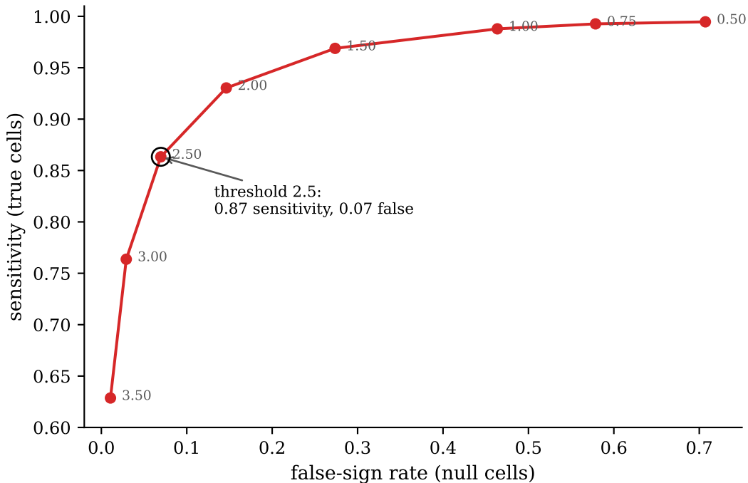
The gate trades sensitivity for false-sign control
