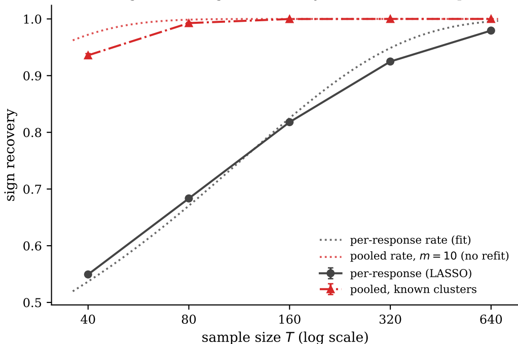
Pooling reaches sign consistency at far smaller samples
