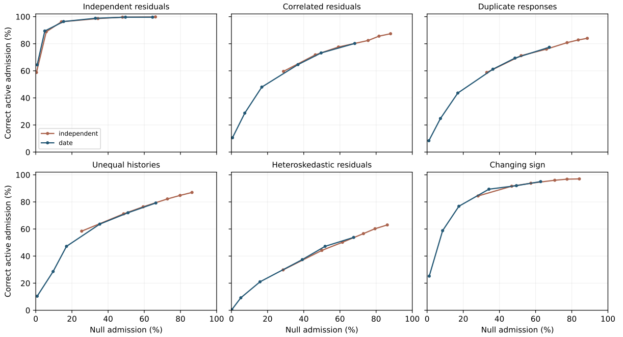
Figure 6: Revised gate trade-offs at EWMA span 60. Each panel uses 500 paired replications and thresholds 0.5, 0.75, 1, 1.5, 2 and 3. Smaller null admission can trade off against active recovery; neither axis alone establishes superiority.
