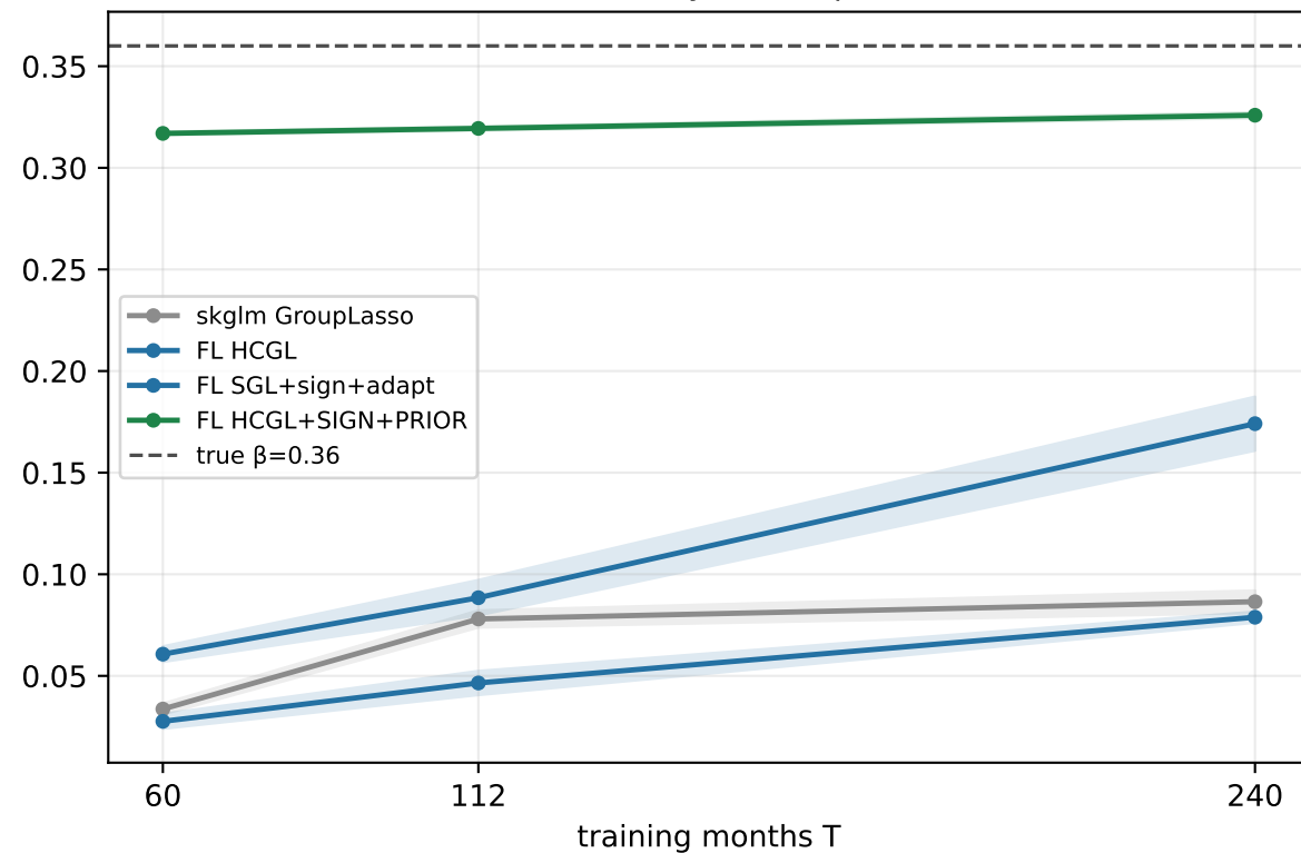
credit recovery vs sample size
