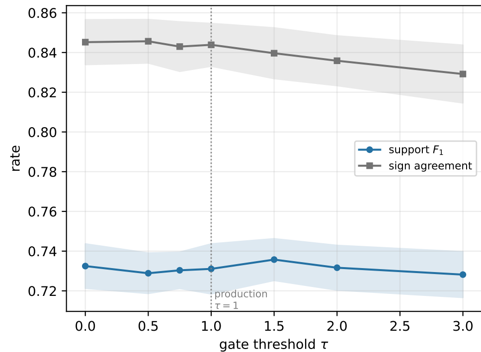
Selection quality is flat across \tau
