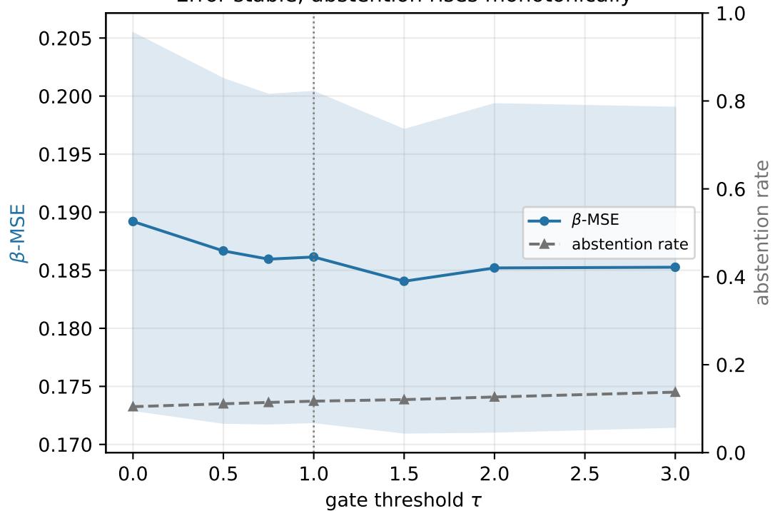
Error stable; abstention rises monotonically
