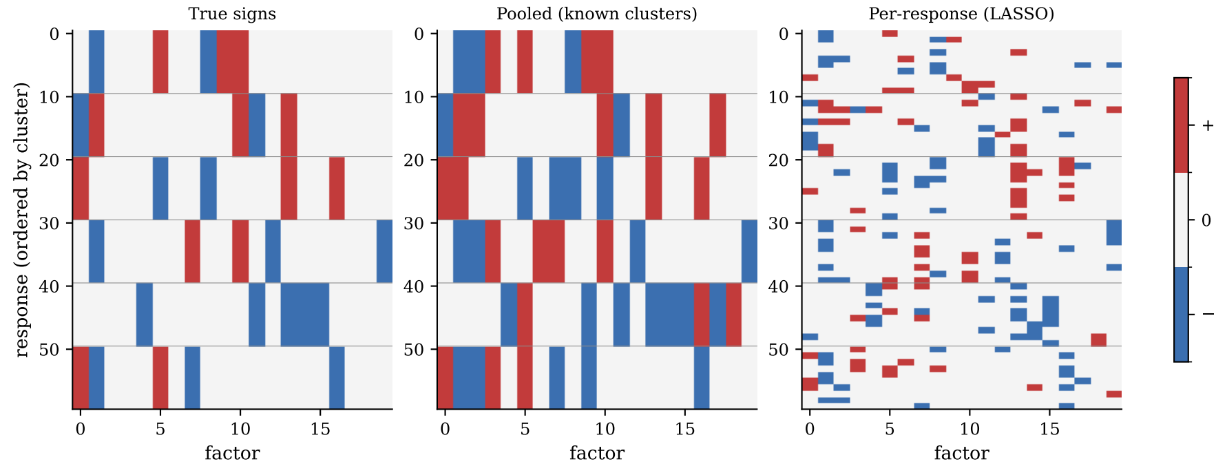
Pooling suppresses spurious within-cluster sign alternations ( R^2=0.2 , threshold 2.0)
