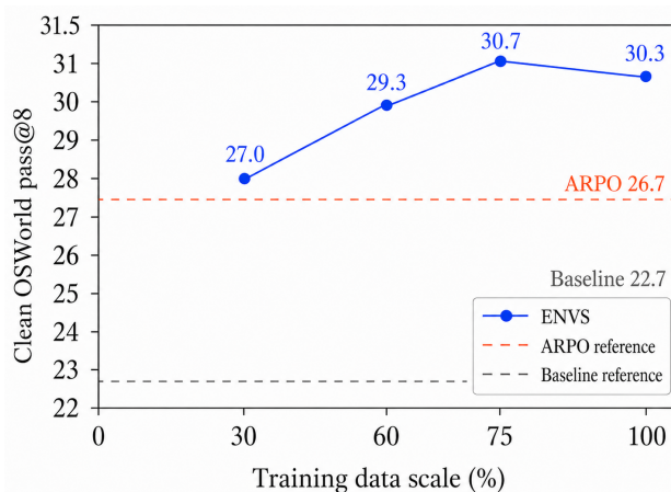
Figure 4: Clean OSWORLD pass@8 as a function of ENVs training data volume. The 30% subset already matches ARPO-clean, while gains saturate near the full dataset.
