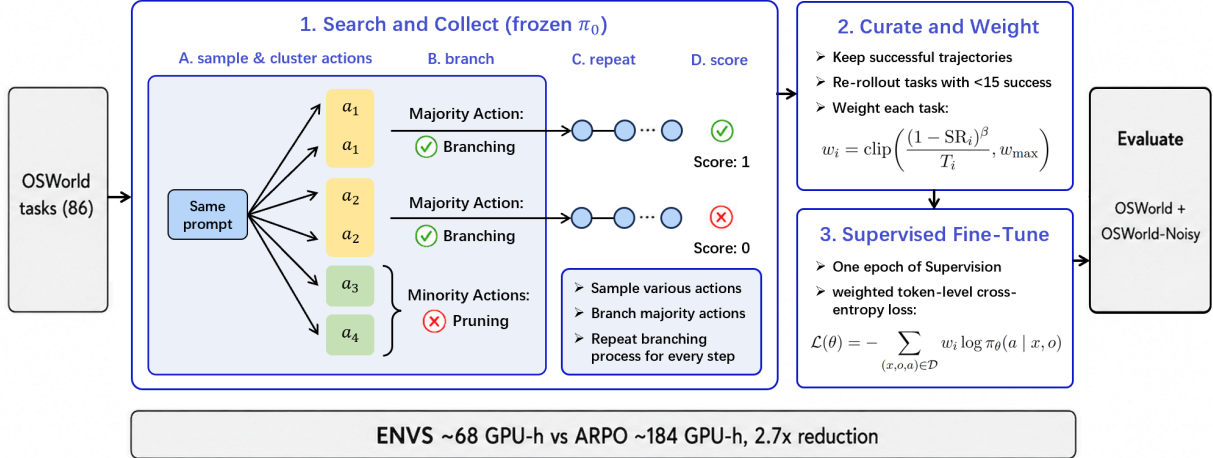
Figure 2: ENVIS pipeline overview. ENVIS uses environment-native tree search to collect verified successful trajectories from OSWORLD, curates them through filtering, weighting, and deduplication, and trains the agent with one-epoch SFT before evaluation on clean and noisy benchmarks.
