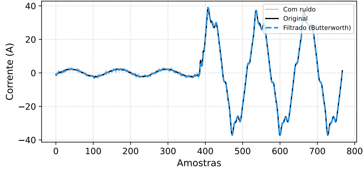
Butterworth — Ordem 3 | f_c = 1100 Hz RMSE = 0.3210 | \Delta SNR = 5.4 dB
