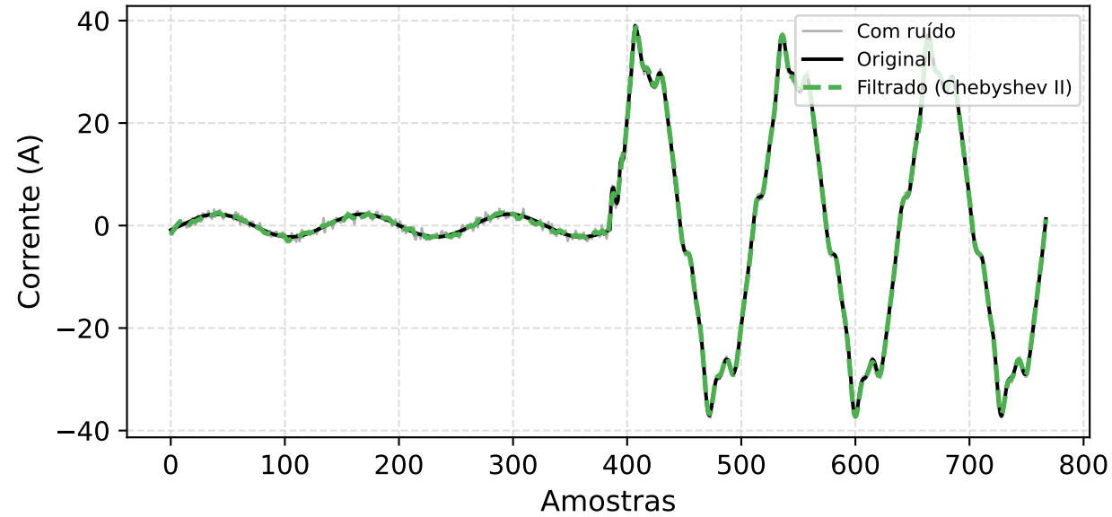
Chebyshev II ★ — Ordem 3 | f_c = 2700 Hz RMSE = 0.3206 | \Delta SNR = 5.4 dB
