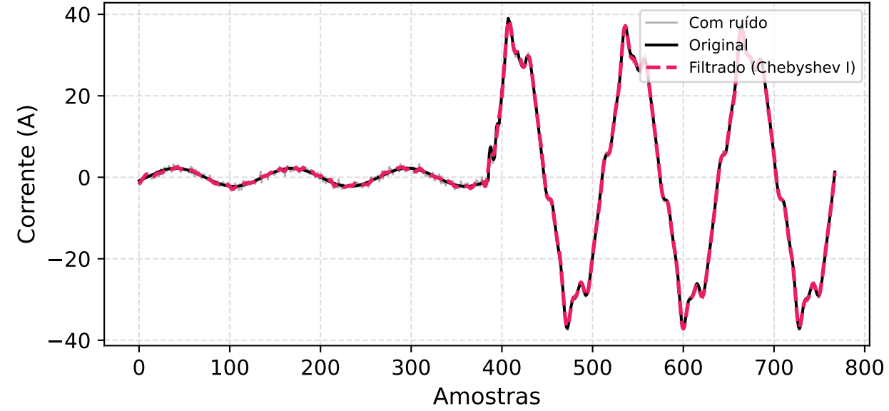
Chebyshev I — Ordem 3 | f_c = 700 Hz RMSE = 0.3260 | \Delta SNR = 5.2 dB
